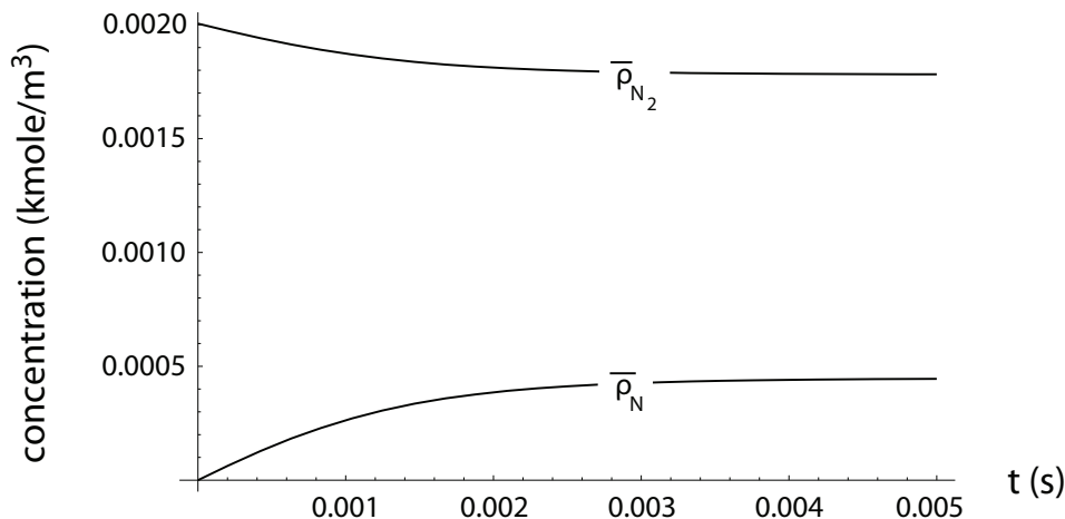
Figure 4.3: \bar{p}_{N_2}(t) and \bar{p}_N(t) in isothermal, isochoric nitrogen dissociation problem.
