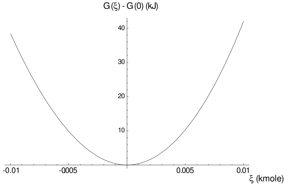
Figure 5.1: Gibbs free energy variation as mixture composition is varied maintaining element conservation for mixture of \text{H}_2 , \text{O}_2 , \text{H}_2\text{O} , \text{OH} , \text{H} , and \text{O} at T = 3000 \text{ K} , P = 100 \text{ kPa} .
