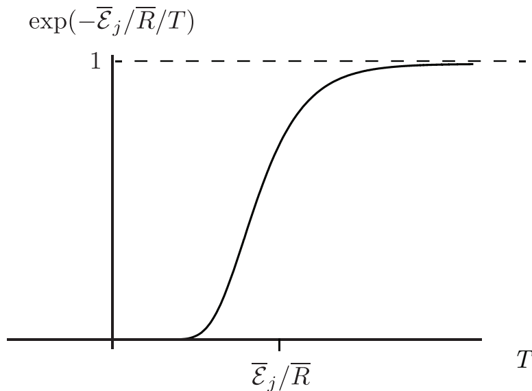
Figure 1.1: Sketch of \exp(-\bar{\mathcal{E}}_j/\bar{R}/T) versus T ; transition occurs at T \sim \bar{\mathcal{E}}_j/\bar{R} .
