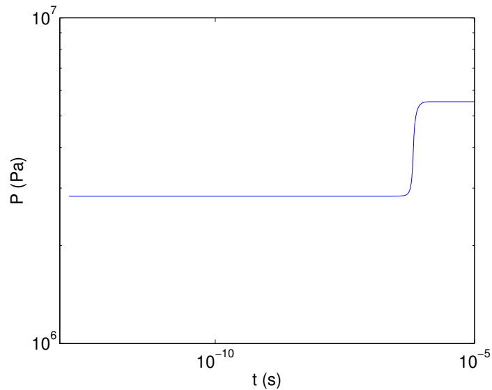
Figure 1.17: Plot of P(t) , for adiabatic, isochoric combustion of a mixture of 2\text{H}_2 + \text{O}_2 + 3.76\text{N}_2 initially at T_o = 1542.7 K, P_o = 2.8323 \times 10^6 Pa.
