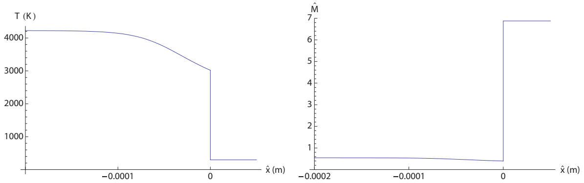
Figure 10.13: ZND structure of T(\hat{x}) and \hat{M}(\hat{x}) for strong D = 2800 \text{ m/s} > D_{CJ} for one-step irreversible reaction for \text{H}_2/\text{air} -based parameters of Table 10.1.
