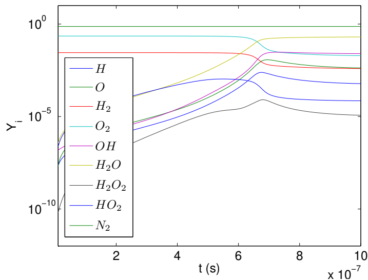
Figure 1.18: Plot near thermal explosion time of Y_{\text{H}_2}(t) , Y_{\text{H}}(t) , Y_{\text{O}}(t) , Y_{\text{O}_2}(t) , Y_{\text{OH}}(t) , Y_{\text{H}_2\text{O}}(t) , Y_{\text{HO}_2}(t) , Y_{\text{H}_2\text{O}_2}(t) , Y_{\text{N}_2}(t) , for adiabatic, isochoric combustion of a mixture of 2\text{H}_2 + \text{O}_2 + 3.76\text{N}_2 initially at T_o = 1542.7 K, P_o = 2.8323 \times 10^6 Pa.
