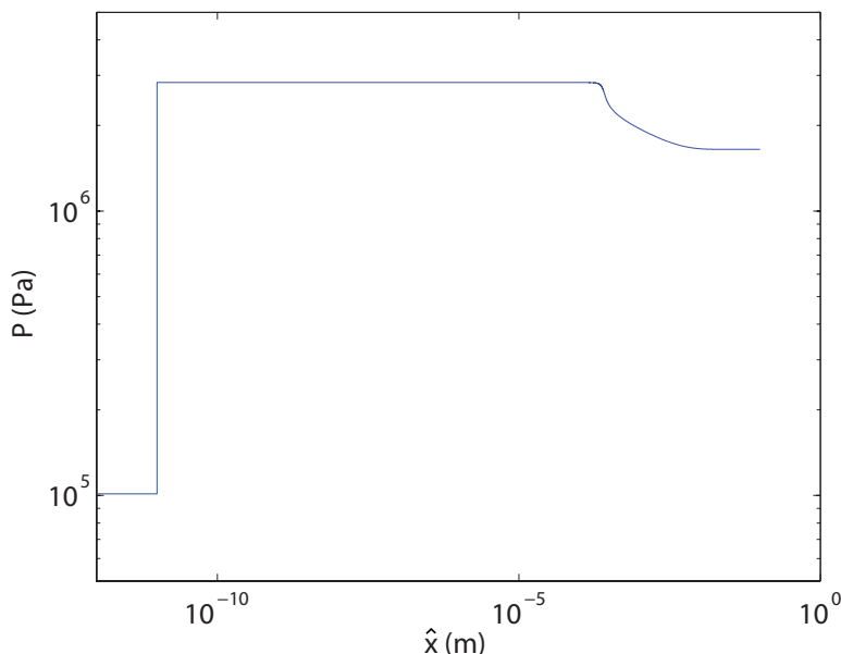
Figure 10.29: Detailed kinetics ZND structure of pressure for near CJ detonation, D_{CJ} \sim D = 1979.70 m/s, in 2\text{H}_2 + \text{O}_2 + 3.76\text{N}_2 , P_o = 1.01325 \times 10^5 Pa, T_o = 298 K, T_s = 1542.7 K P_s = 2.83280 \times 10^6 Pa.
