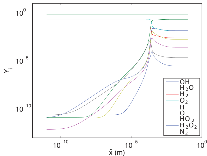
Figure 10.28: Detailed kinetics ZND structure of species mass fractions for near CJ detonation, D_{CJ} \sim D = 1979.70 m/s, in 2H_2 + O_2 + 3.76N_2 , P_o = 1.01325 \times 10^5 Pa, T_o = 298 K, T_s = 1542.7 K, P_s = 2.83280 \times 10^6 Pa.
