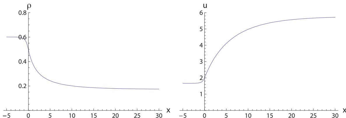
Figure 9.3: Dimensionless density \rho and fluid particle velocity u as functions of distance for a burner-stabilized premixed laminar flame, T_{IG} = 0.2 .
