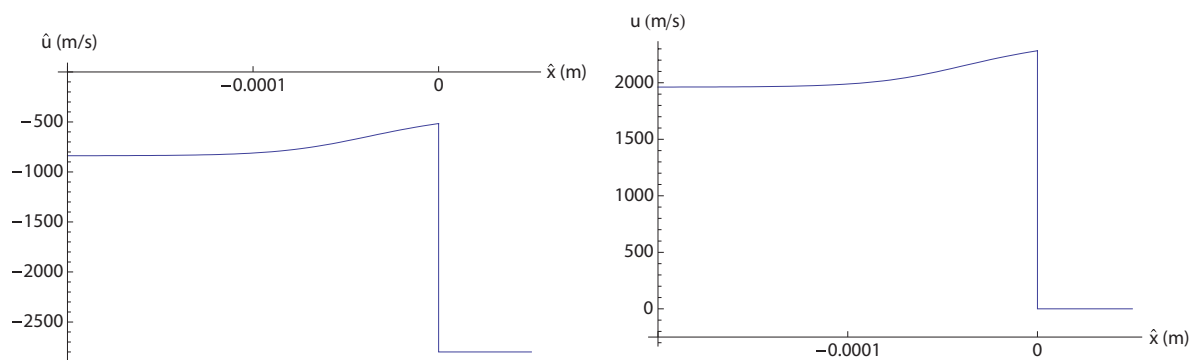
Figure 10.12: ZND structure of wave frame-based fluid particle velocity \hat{u}(\hat{x}) and laboratory frame-based fluid particle velocity u(\hat{x}) for strong D = 2800 m/s > D_{CJ} for one-step irreversible reaction for H 2 /air-based parameters of Table 10.1.
