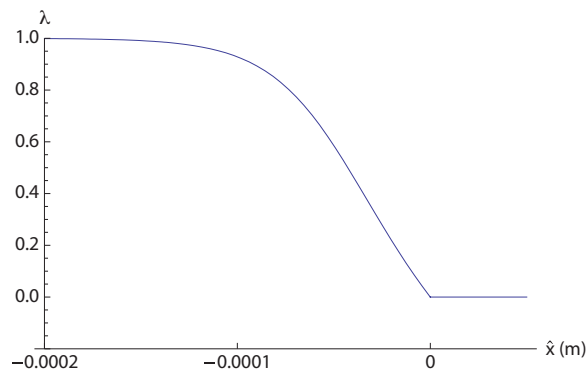
Figure 10.14: ZND structure of \lambda(\hat{x}) for strong D = 2800 \text{ m/s} > D_{CJ} for one-step irreversible reaction for \text{H}_2/\text{air} -based parameters of Table 10.1.
