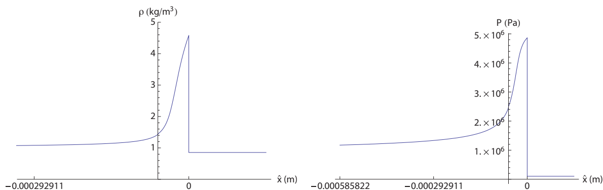
Figure 10.24: ZND structure of \rho(\hat{x}) and P(\hat{x}) for weak D = 2616.5 m/s = \tilde{D} for two-step irreversible reaction with parameters of Table 10.3.
