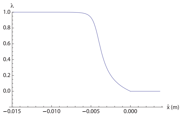
Figure 10.9: ZND structure of \lambda(\hat{x}) for D = D_{CJ} = 1991.1 m/s for one-step irreversible reaction for \text{H}_2/\text{air} -based parameters of Table 10.1.
