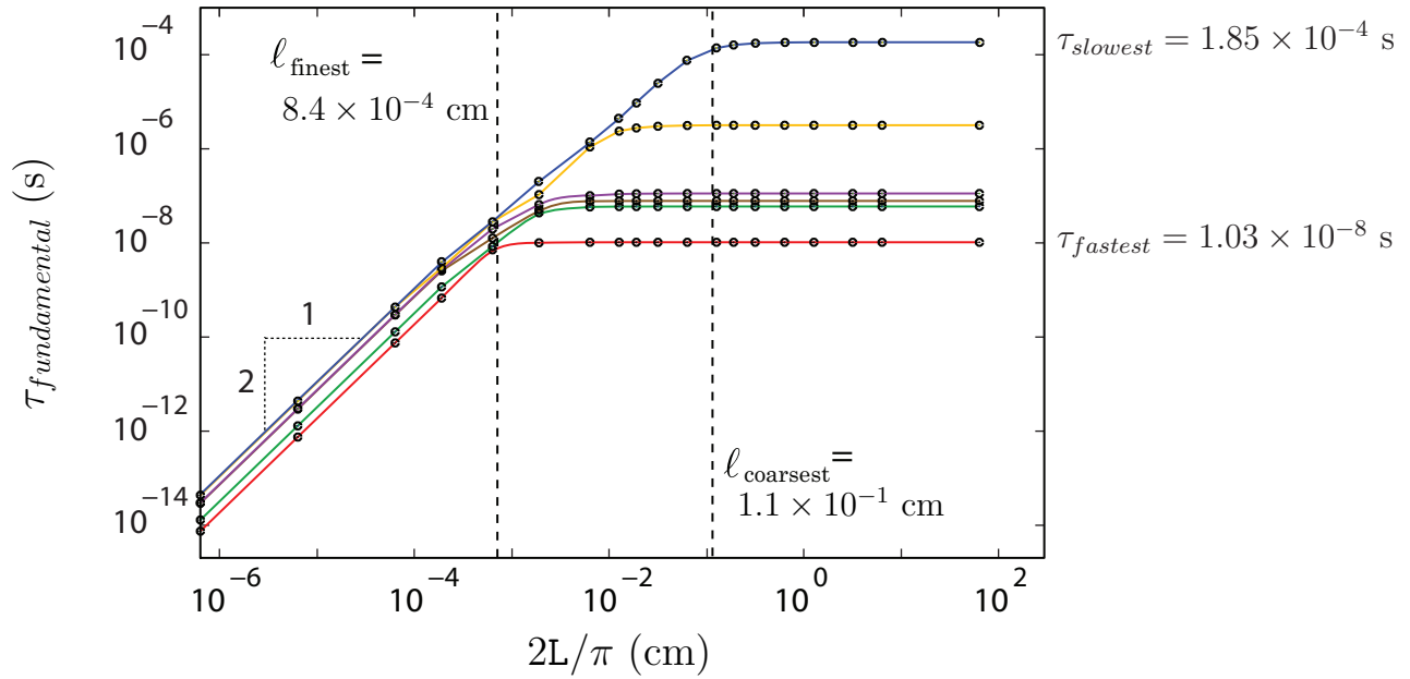
Figure 7.2: Time scales associated with the fundamental modes for a nine-species, nineteen step stoichiometric, p = 1 atm, T_o = 800 K hydrogen–air reaction–advection–diffusion system versus the length 2L/\pi .
