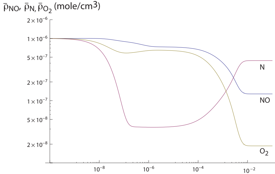
Figure 5.4: NO, N, and O 2 concentrations versus time for T = 6000 K, extended Zel'dovich mechanism.
