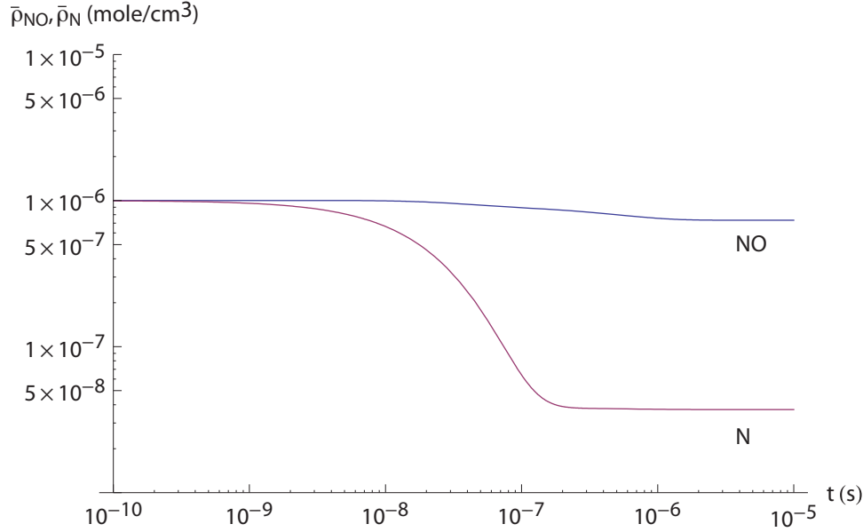
Figure 1.8: NO and N concentrations versus time for T = 6000 K, P = 2.4942 \times 10^6 dyne/cm 2 Zel'dovich mechanism.
