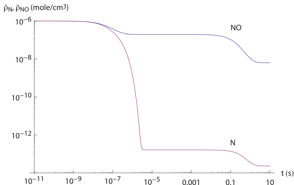
Figure 1.10: \bar{\rho}_{\text{NO}} and \bar{\rho}_{\text{N}} versus time for Zel'dovich mechanism at T = 1500 K, P = 6.23550 \times 10^5 dyne/cm 2 .
