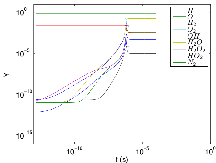
Figure 1.15: Plot of Y_{\text{H}_2}(t) , Y_{\text{H}}(t) , Y_{\text{O}}(t) , Y_{\text{O}_2}(t) , Y_{\text{OH}}(t) , Y_{\text{H}_2\text{O}}(t) , Y_{\text{HO}_2}(t) , Y_{\text{H}_2\text{O}_2}(t) , Y_{\text{N}_2}(t) , for adiabatic, isochoric combustion of a mixture of 2\text{H}_2 + \text{O}_2 + 3.76\text{N}_2 initially at T_o = 1542.7 K, P_o = 2.8323 \times 10^6 Pa.
