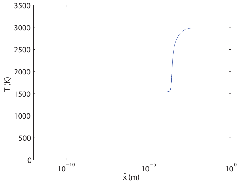
Figure 10.30: Detailed kinetics ZND structure of temperature for near CJ, D_{CJ} \sim D = 1979.70 m/s, detonation in 2\text{H}_2 + \text{O}_2 + 3.76\text{N}_2 , P_o = 1.01325 \times 10^5 Pa, T_o = 298 K, T_s = 1542.7 K, P_s = 2.83280 \times 10^6 Pa. Shock at \hat{x} = 0 artificially translated to \hat{x} = 10^{-11} m.
