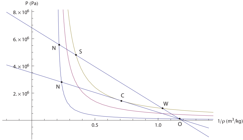
Figure 10.2: Plot of \lambda = 0, 1/2, 1 Hugoniot curves and two Rayleigh lines for D = 2800 m/s, D = 1991.1 m/s and parameters of Table 10.1.
