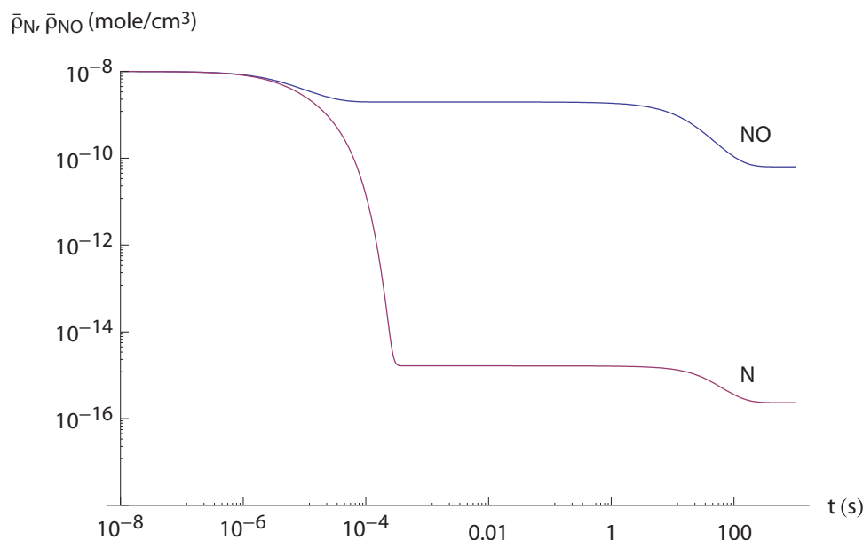
Figure 1.11: \bar{\rho}_{\text{NO}} and \bar{\rho}_{\text{N}} versus time for Zel'dovich mechanism at T = 1500 K, P = 6.2355 \times 10^3 dyne/cm 2 .
