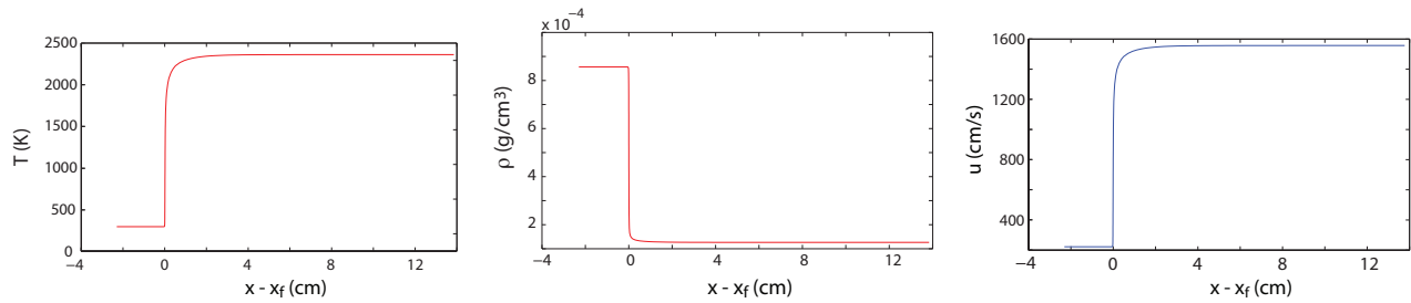
Figure 9.10: Temperature, density, and fluid particle velocity as functions of distance in a premixed laminar flame with detailed \text{H}_2\text{-O}_2\text{-N}_2 kinetics.
