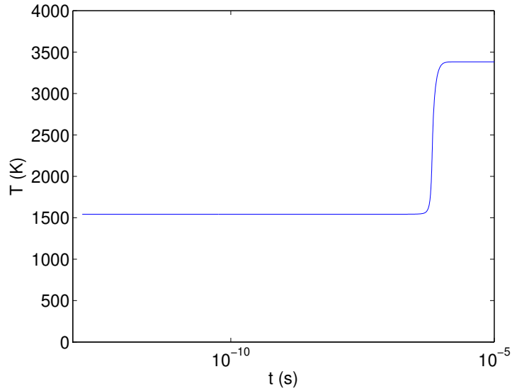
Figure 1.16: Plot of T(t) , for adiabatic, isochoric combustion of a mixture of 2\text{H}_2 + \text{O}_2 + 3.76\text{N}_2 initially at T_o = 1542.7 K, P_o = 2.8323 \times 10^6 Pa.
