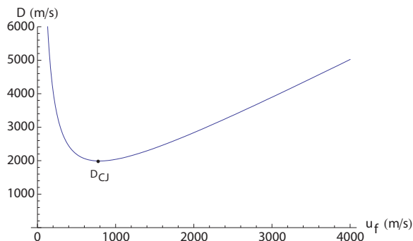
Figure 10.3: Plot of detonation wave speed D versus piston velocity u_f ; parameters from Table 10.1 loosely model \text{H}_2 -air detonation.
