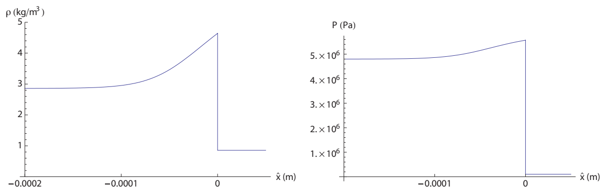
Figure 10.11: ZND structure of \rho(\hat{x}) and P(\hat{x}) for strong D = 2800 m/s > D_{CJ} for one-step irreversible reaction for H 2 /air-based parameters of Table 10.1.
