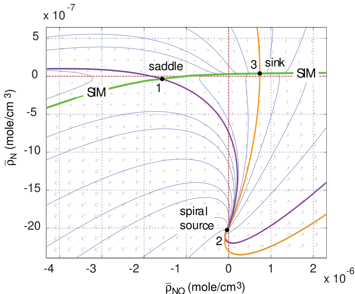
Figure 1.9: NO and N phase portraits for T = 6000 K, P = 2.4942 \times 10^6 dyne/cm 2 Zel'dovich mechanism.
