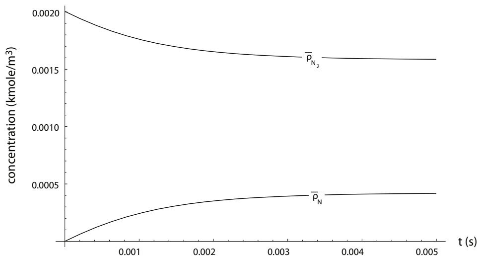
Figure 4.5: \bar{\rho}_{N_2}(t) and \bar{\rho}_N(t) in isobaric, isothermal nitrogen dissociation problem.
