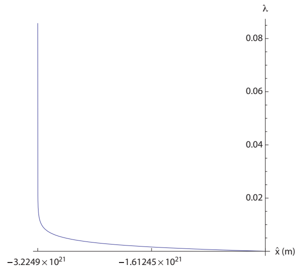
Figure 10.15: ZND structure of \lambda(\hat{x}) for unshocked, weak D = 2800 \text{ m/s} > D_{CJ} for one-step irreversible reaction for \text{H}_2/\text{air} -based parameters of Table 10.1. The galactic distance scales are far too large to be realistic representations of reality!
