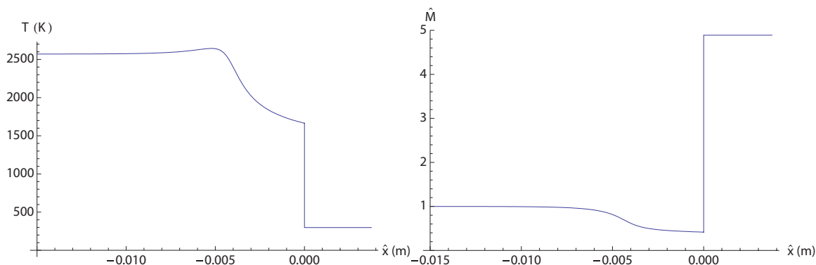
Figure 10.8: ZND structure of T(\hat{x}) and wave frame-based Mach number \hat{M} for D = D_{CJ} = 1991.1 m/s for one-step irreversible reaction for \text{H}_2/\text{air} -based parameters of Table 10.1.
