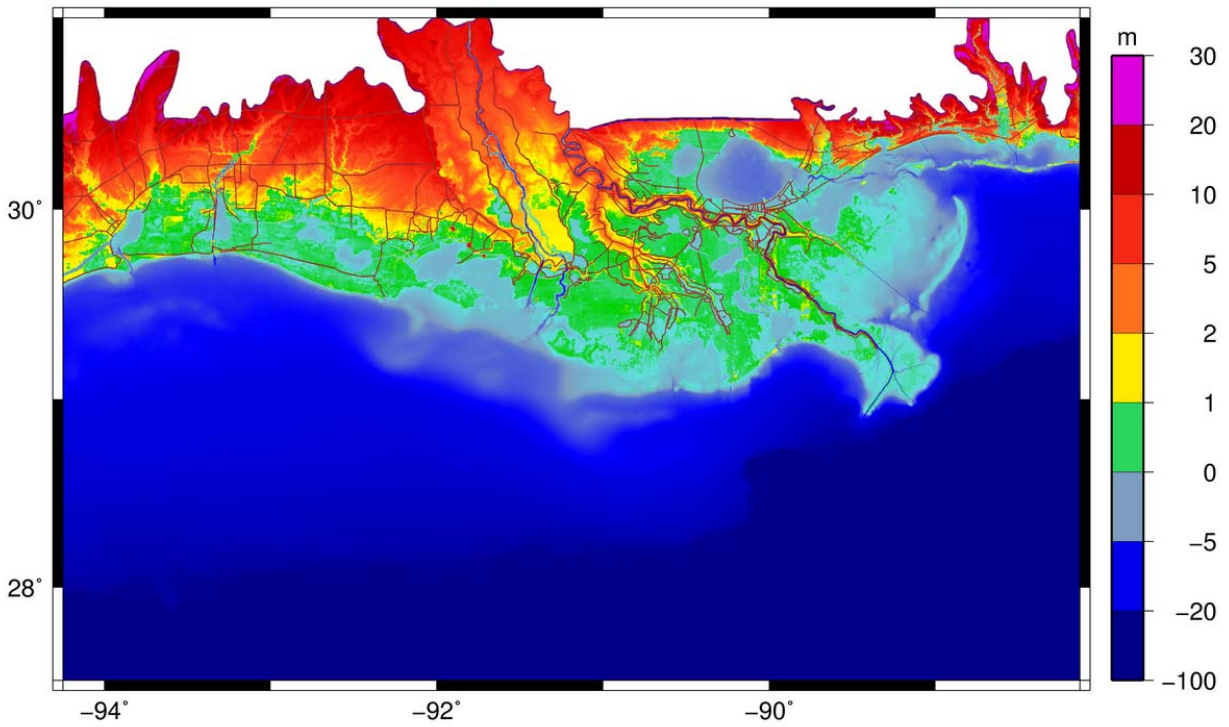
Figure 3: ADCIRC SL15 bathymetry and topography (m), relative to NAVD88 (2004.65), for southern Louisiana.
