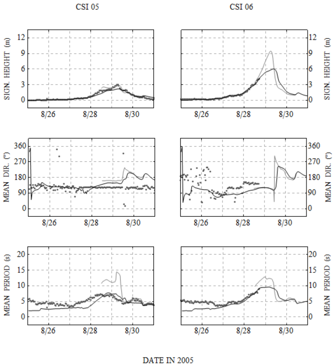
Figure 14: Hurricane Katrina significant wave heights (m); mean wave directions ( ^{\circ} ), measured clockwise from geographic north; and mean wave periods (s) at two CSI buoys. The measured data is shown with black dots, the modeled SWAN results are shown with black lines, and the modeled WAM/STWAVE results are shown with gray lines. The CSI buoy data was collected by WAVCIS ( http://www.wavcis.lsu.edu ).
