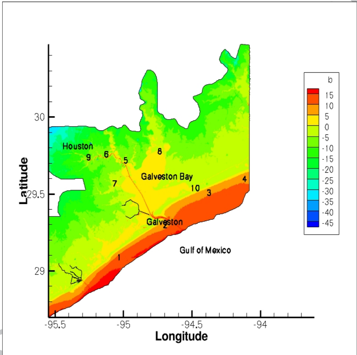
Figure 4: Bathymetry (m) in Galveston Bay and the surrounding area. The Houston Ship Channel is the narrow line that runs through Galveston Bay from Galveston to Houston. Numbers indicate locations of hydrographs for Hurricane Ike simulations.
