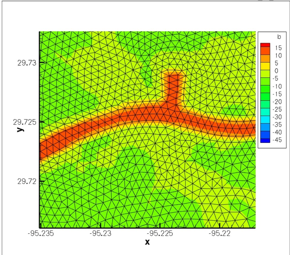
Figure 13: Bathymetry with finite element mesh overlaid along a stretch of the Houston Ship Channel near Manchester. Bathymetry ( b ) is in meters. Note that a string of nodes follows the deepest part of the channel and in some places the channel is split across two elements.
