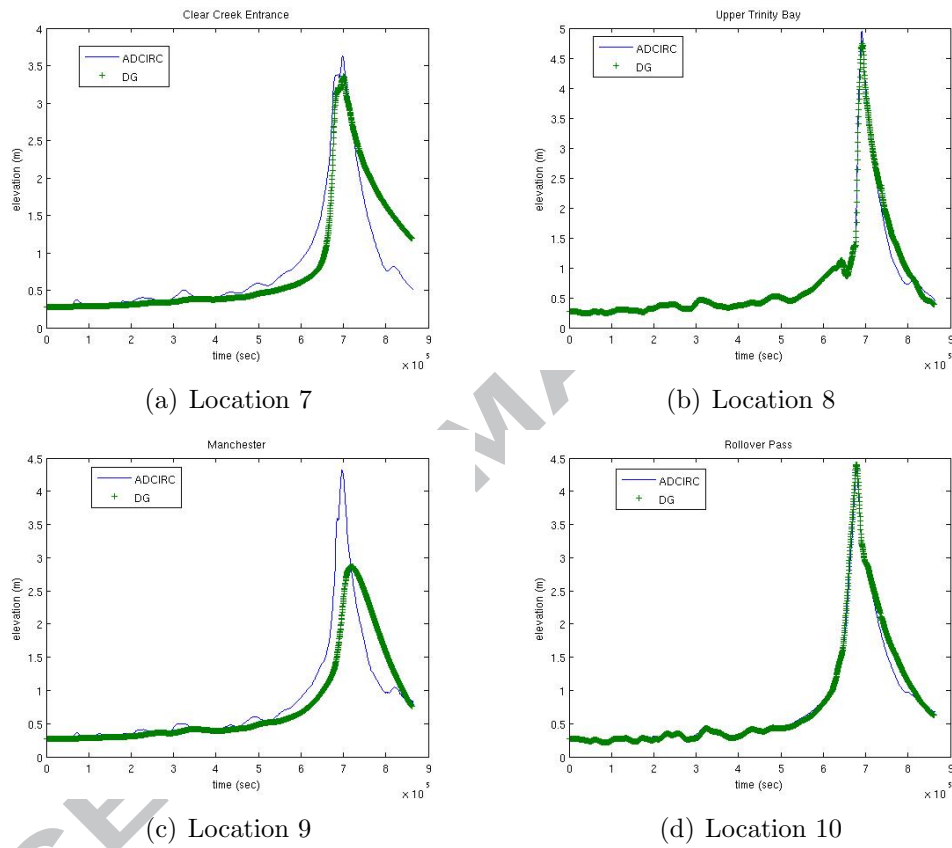
Figure 10: Hydrographs of ADCIRC and DG solutions locations 7-10 for Hurricane Ike. Water levels are in meters relative to NAVD88.
