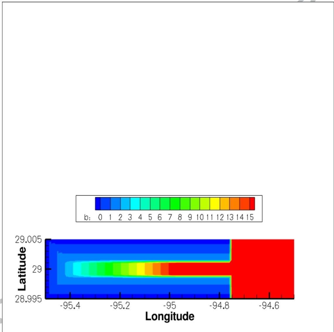
Figure 5: Model channel domain. Bathymetry is in meters.
