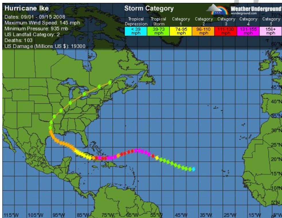
Figure 3: Track of Hurricane Ike ( http://www.wunderground.com )
