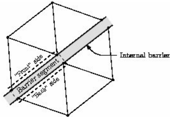
Figure 1: An internal barrier and surrounding elements in a domain. Edge pairs on either side of the barrier are identified as barrier segments.
