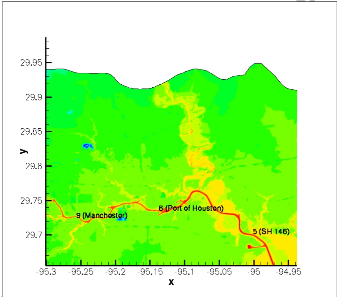
Figure 12: Closer view of the upper reaches of the Houston Ship Channel, which shows measurement locations 5 (SH 146 bridge), 6 (Port of Houston) and 9 (Manchester). Colors represent bathymetric depth.
