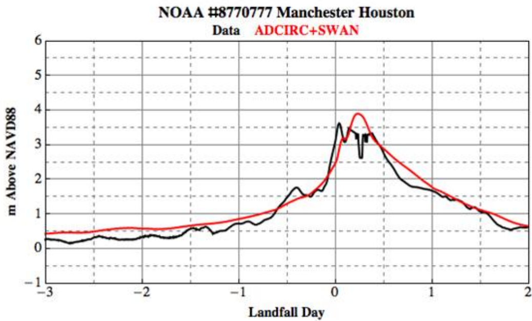
Figure 11: Comparison of ADCIRC+SWAN computed water levels with NOAA gauge data at location 9 (Manchester, Houston, Texas).
