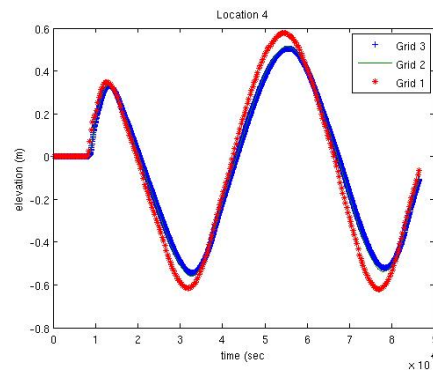
(f) Location 4: Slope limiter 3 convergence
