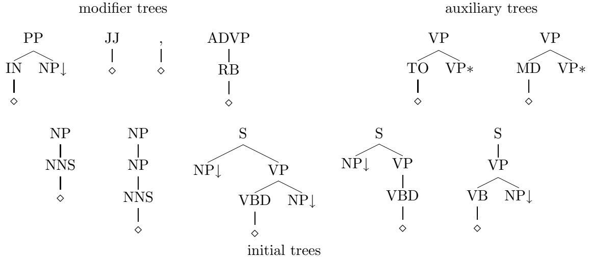
Figure 3: A few of the more frequently-occurring tree templates. \diamond marks where the lexical anchor is inserted.
