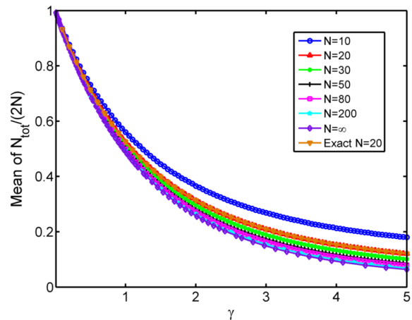
FIG. 1. Mean number of stationary points as a function of \gamma .
