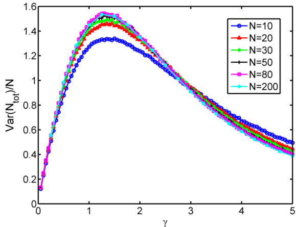
FIG. 3. Variance of the number of stationary points as a function of \gamma .
