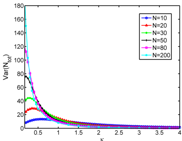
FIG. 4. Variance of the number of stationary points as a function of \kappa .
