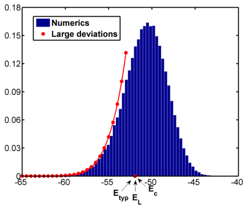
FIG. 6. Probability density of E_{\min} for \gamma = 2 and N = 50 .
