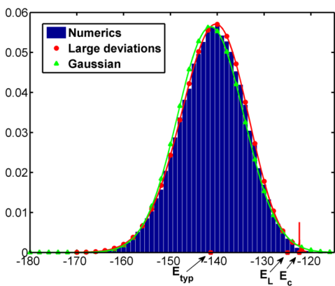
FIG. 7. Probability density of E_{\min} for \sigma = 1 and N = 100 .
