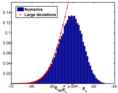
FIG. 9. Probability density of E_{\min} for \kappa = 1 and N = 50 .
