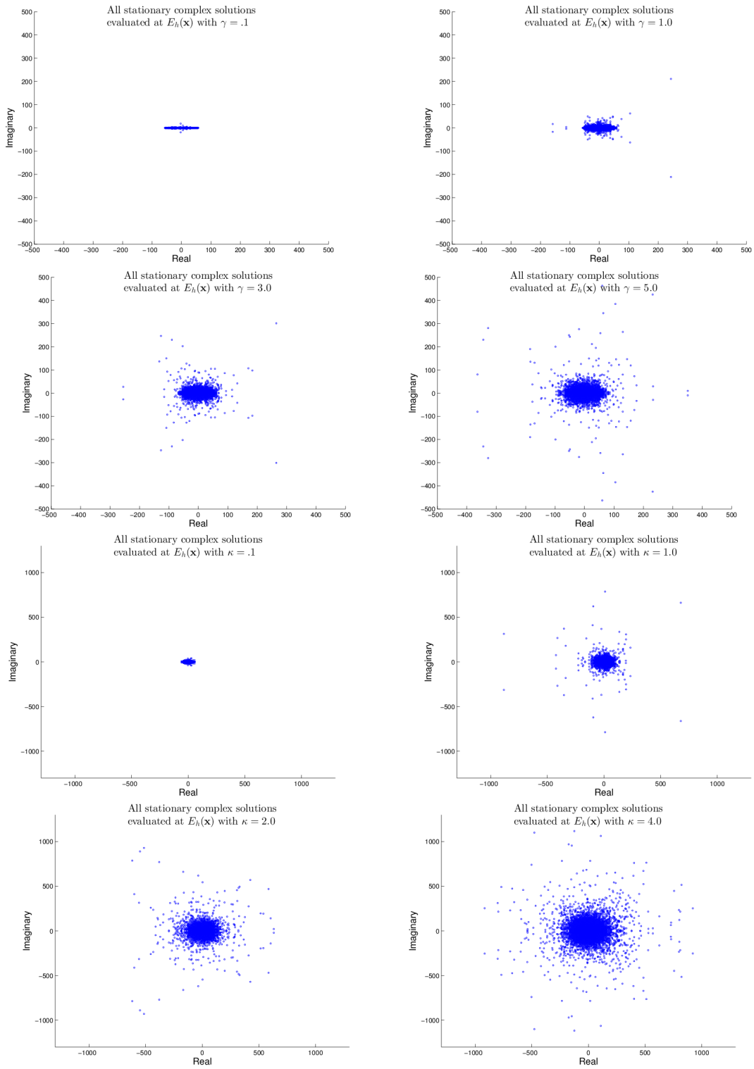
FIG. 10. Plots of the real and imaginary parts of the energy function E_h(\mathbf{x}) evaluated at the complex stationary points for different values of \gamma and \kappa .
