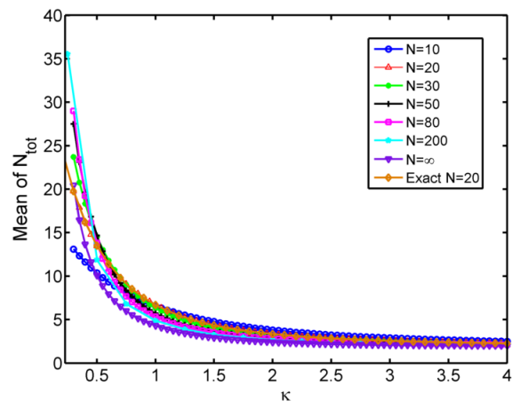
FIG. 2. Mean number of stationary points as a function of \kappa .
