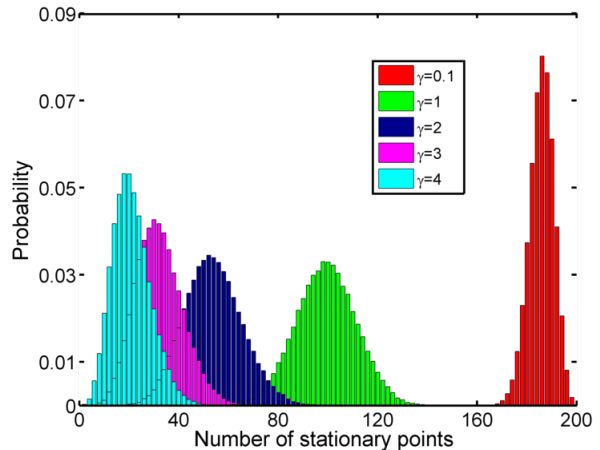
FIG. 5. Probability densities of the number of stationary points for different values of \gamma .
