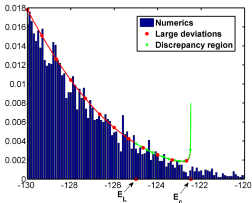
FIG. 8. Probability density of E_{\min} near the critical energy, again with \sigma = 1 and N = 100 .
