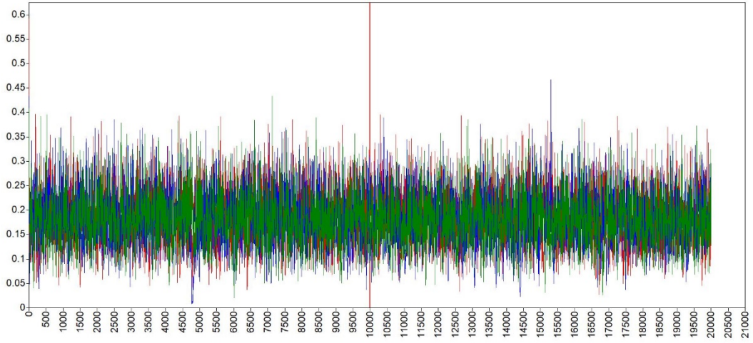
\text{Var}(u_{a_i})
