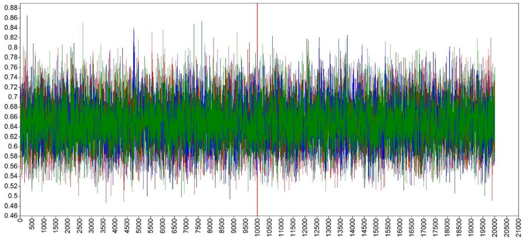
\text{Var}(e_M)
