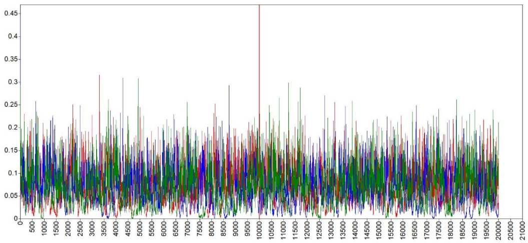
\text{Var}(u_{c_i})
