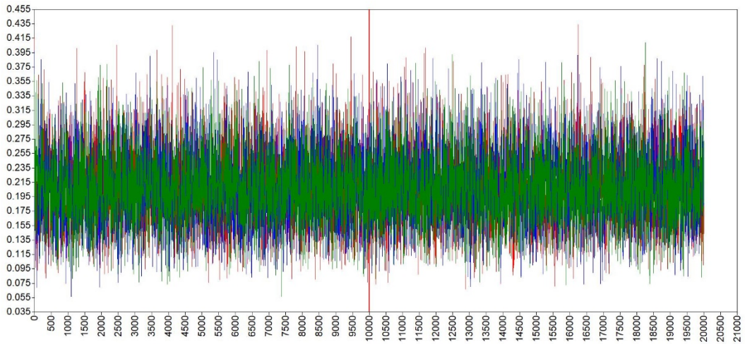
\text{Var}(u_{b_i})
