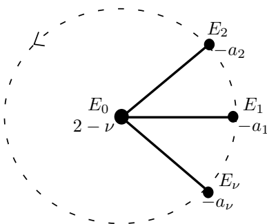
Figure 2: The resolution graph of a “polygonal” singularity
