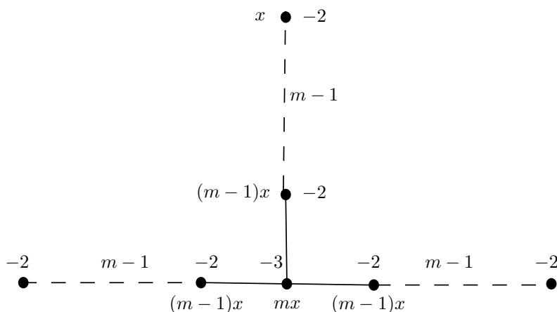
Figure 1: The resolution graph of the rational singularity (X, 0)
