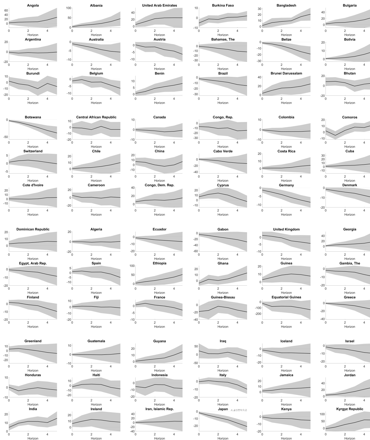
Figure D1: Global Temperature Local Projection Impulse Responses
