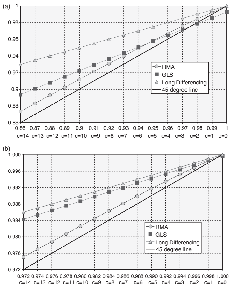
Figure 3. Comparison of inconsistencies among \hat{\rho}_{\text{RMA}} , \hat{\rho}_{\text{GLS}} and \hat{\rho}_{\text{long}} . (a) T=100, N=2,000 ; (b) T=500, N=2,000
