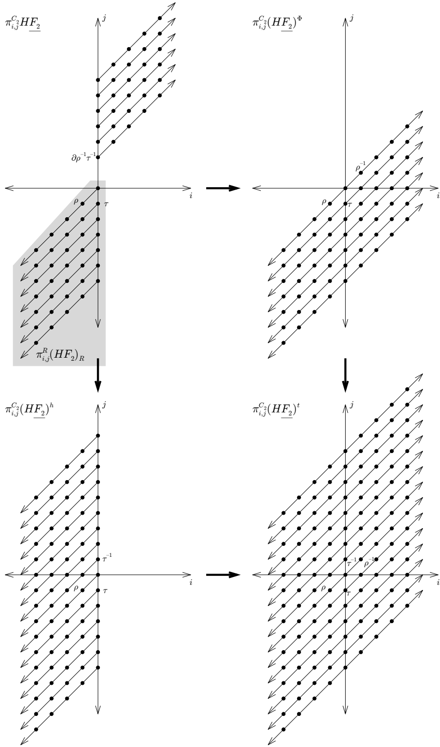
FIGURE 9.1. Computing \pi_{*,*}^{C_2} \underline{HF}_2 from \pi_{*,*}^{\mathbb{R}}(HF_2)_{\mathbb{R}} .
