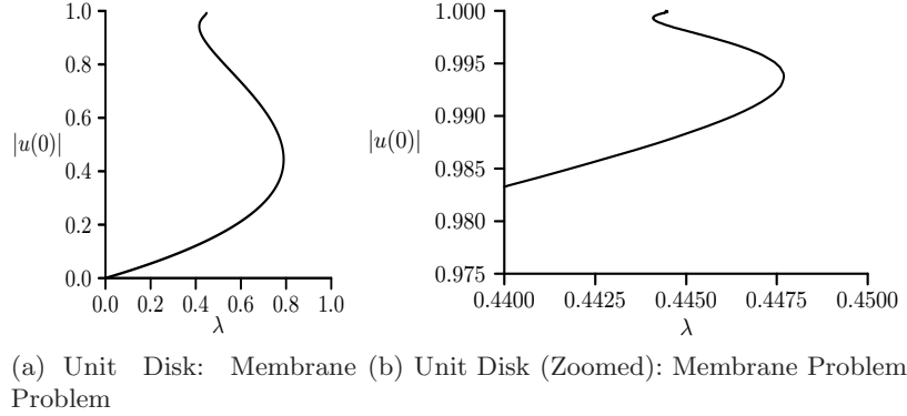
FIGURE 2. Numerical solutions for |u(0)| versus \lambda computed from (1.2) for the unit disk \Omega = \{|x| \leq 1\} in two-dimensions. The magnified figure on the right shows the beginning of the infinite set of fold points
