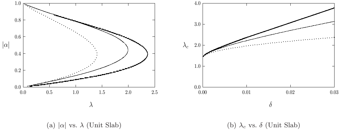
FIGURE 6. Left figure: Plot of numerically computed global bifurcation diagram |\alpha| = |u(1/2)| versus \lambda for (1.1) with \delta = 0.01 (heavy solid curve) compared to the two-term asymptotic result (3.12) (solid curve) and the unperturbed \delta = 0 membrane MEMS result from (1.2) (dashed curve). Right figure: Comparison of numerically computed fold point \lambda_c versus \delta (heavy solid curve) with the two-term (dashed curve) and the three-term (solid curve) asymptotic result from (3.28).
