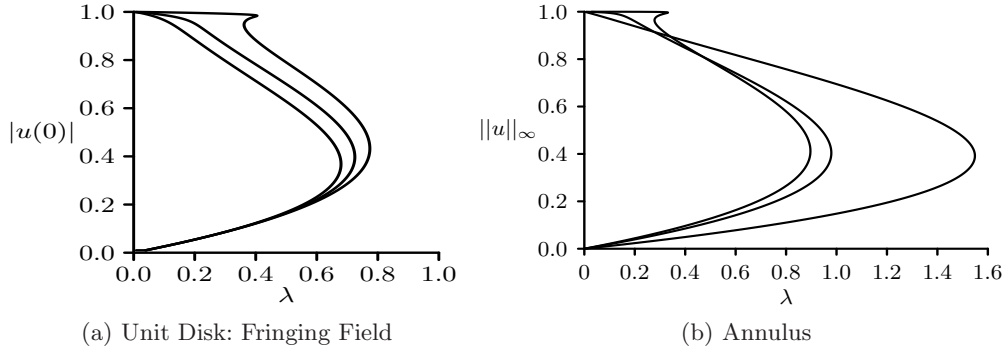
FIGURE 4. Left figure: Numerical solutions for |u(0)| versus \lambda computed from the fringing-field problem (1.4) for the unit disk \Omega = \{|x| \leq 1\} with, from left to right, \delta = 1, 0.5, 0.1 . Right figure: Numerical solutions for |u|_\infty versus \lambda computed from (1.5) in the annulus \delta < r < 1 with, from left to right, \delta = 0.00001, 0.001, 0.1 .
