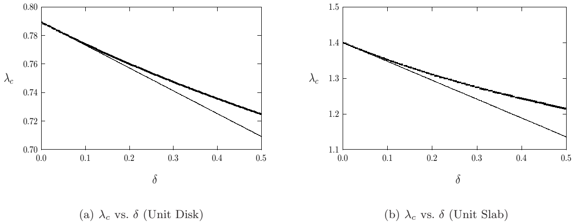
FIGURE 9. Left figure: Comparison of full numerical result for \lambda_c versus \delta (heavy solid curve) for the fringing-field problem computed from (1.4) with the two-term asymptotic result (6.5) (solid curve) for the unit disk. Right figure: A similar comparison for the unit slab.
