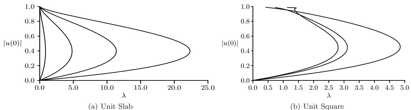
FIGURE 5. Numerical solutions of (1.1) for the slab 0 < x < 1 (left figure) and the unit square for several values of \delta . From left to right the solution branches correspond to \delta = 0.1, 1.0, 2.5, 5.0 (left figure) and \delta = 0.0001, 0.001, 0.01 (right figure).
