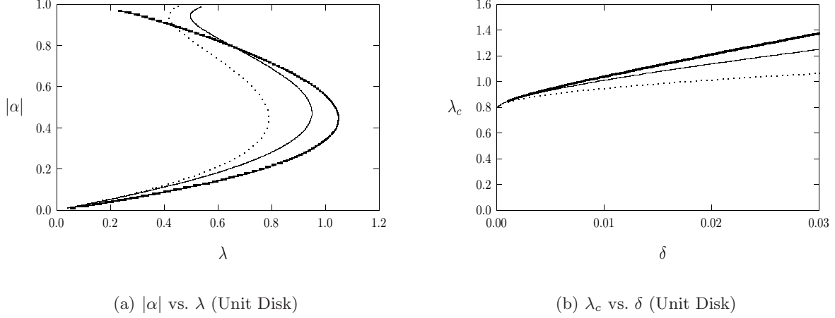
FIGURE 7. Left figure: Plot of numerically computed global bifurcation diagram |\alpha| = |u(0)| versus \lambda for (1.1) with \delta = 0.01 (heavy solid curve) compared to the two-term asymptotic result (4.20) (solid curve) and the unperturbed \delta = 0 membrane MEMS result from (1.2) (dashed curve). Right figure: Comparison of numerically computed fold point \lambda_c versus \delta (heavy solid curve) with the two-term (dashed curve) and the three-term (solid curve) asymptotic result from (4.19).
