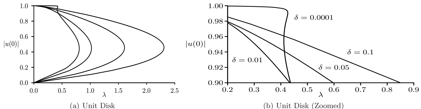
FIGURE 3. Numerical solutions of (1.1) for the unit disk \Omega = \{|x| \leq 1\} for several values of \delta . From left to right the solution branches correspond to \delta = 0.0001, 0.01, 0.05, 0.1 . The figure on the right is a magnification of a portion of the left figure.
