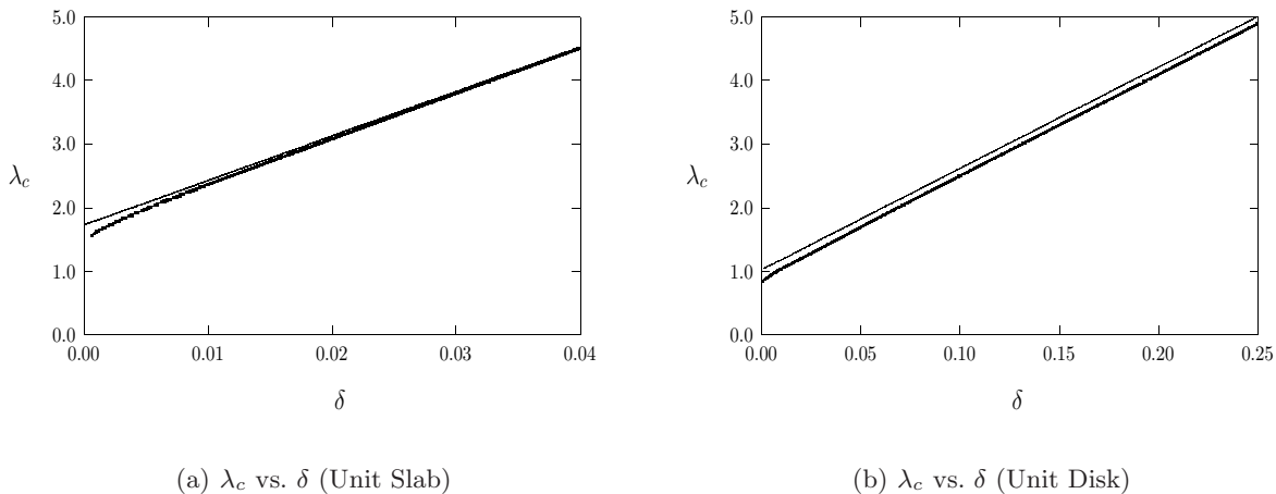
FIGURE 8. Comparison of full numerical result for \lambda_c versus \delta (heavy solid curves) computed from (1.1) with the two-term asymptotic results (5.8) (solid curves) for the unit slab (left figure) and the unit disk (right figure).
