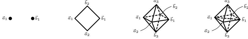
Figure 2: The first three pictures depict the images of Y_1 , Y_2 , and Y_3 in \mathfrak{YB}_g(\mathbb{Z}/2) . The fourth picture indicates a nullhomotopy of Y_3 in \widehat{\mathfrak{YB}}_g(\mathbb{Z}/2) using simplices of intersection type.
