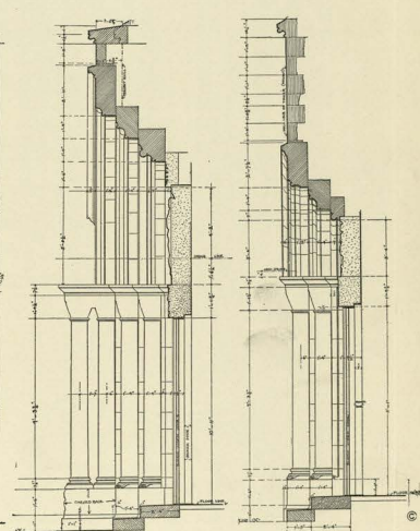
SECTION, CENTER DOOR
