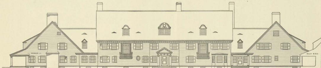
COURT ELEVATION OF HOUSE
