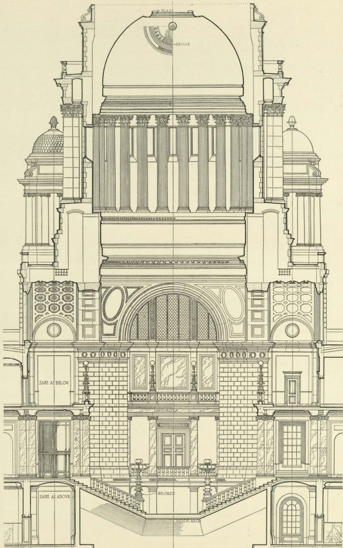
THE RHODE ISLAND STATE CAPITOL, PROVIDENCE, R. I. SECTION THROUGH ROTUNDA 1895 - 1893
