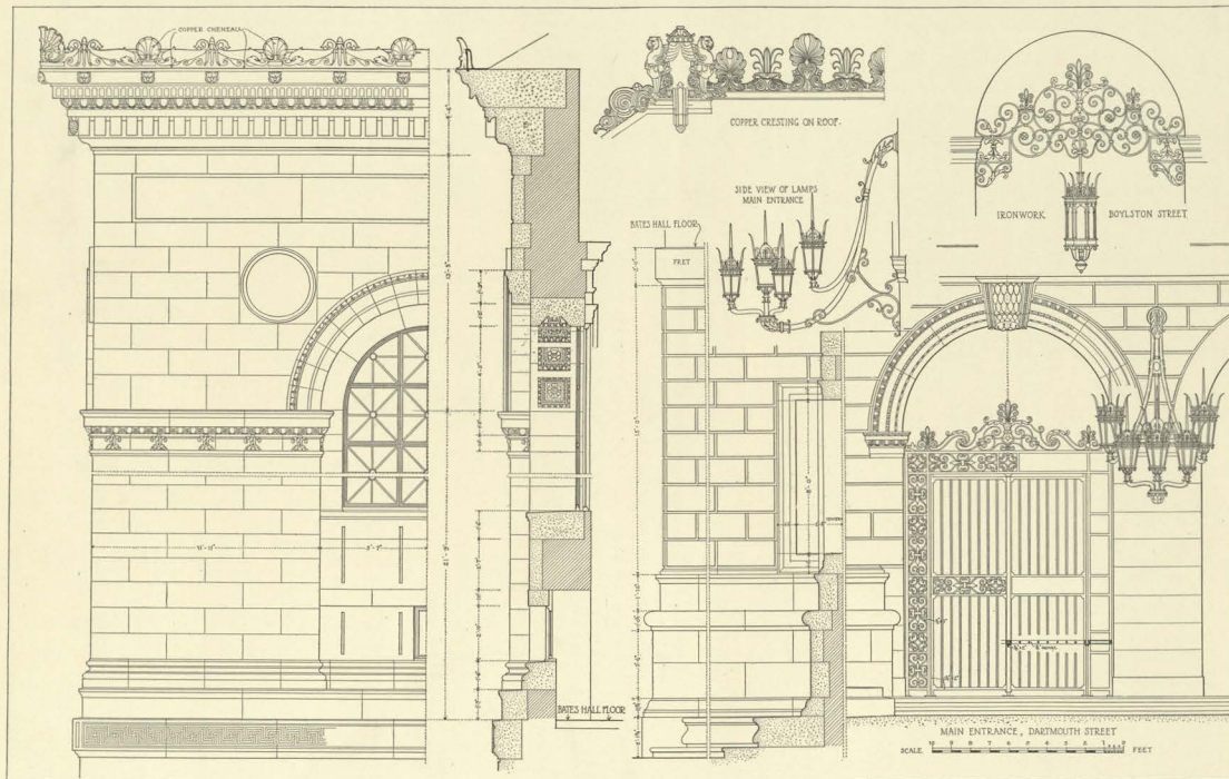
EXTERIOR DETAILS BOSTON PUBLIC LIBRARY, BOSTON, MASS. 1898
