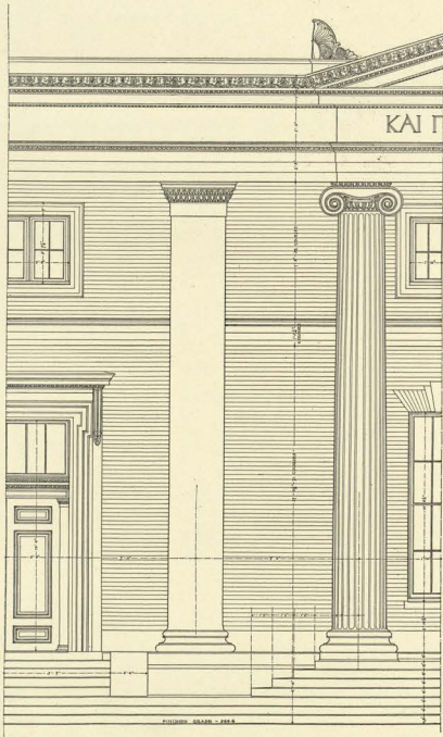
DETAIL CENTRAL PORTION, ACADEMIC BUILDING UNIVERSITY OF VIRGINIA, CHARLOTTESVILLE, VA. 1898
