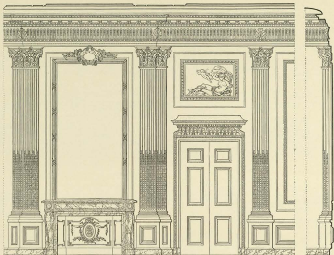
DETAILS OF EAST ROOM
