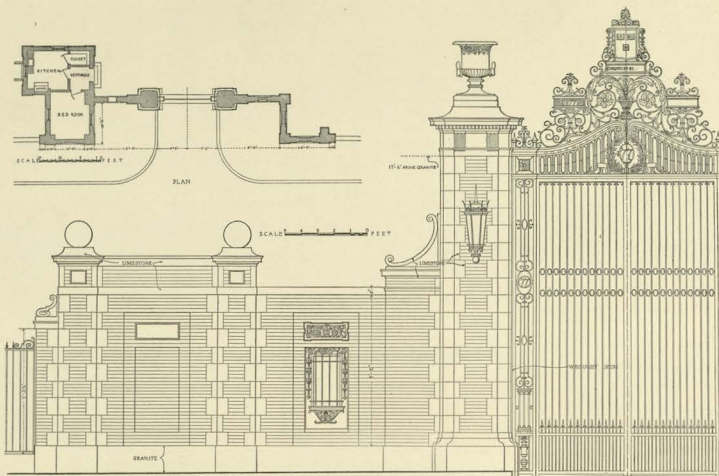
FRONT ELEVATION CLASS OF 1877
