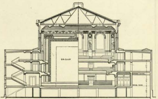
TRANSVERSE SECTIONS
