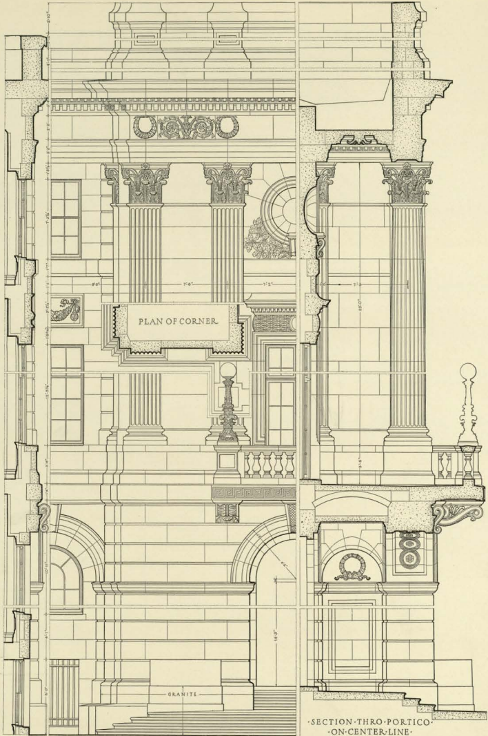
DETAIL OF CENTRAL PORTION OF SOUTH ELEVATION
