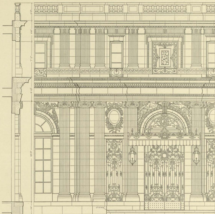
·PORTION OF FACADE AT MAIN ENTRANCE·
