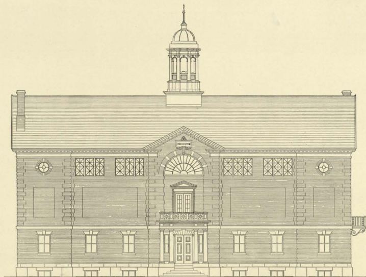
SCALE 0 5 10 15 20 FEET ELEVATION RADCLIFFE COLLEGE GYMNASIUM, CAMBRIDGE, MASS. 1899
