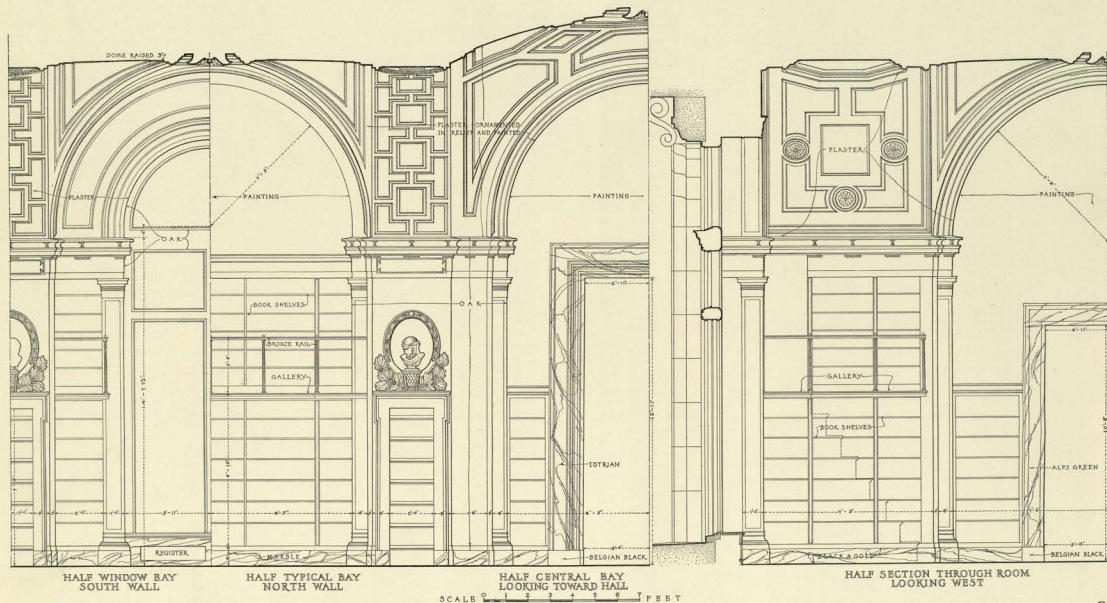
UNIVERSITY CLUB, NEW YORK CITY DETAILS OF THE LIBRARY 1900
