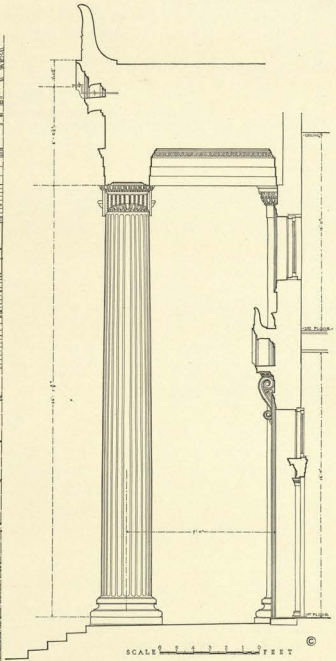
DETAIL CENTRAL PORTION, ACADEMIC BUILDING UNIVERSITY OF VIRGINIA, CHARLOTTESVILLE, VA. 1898
