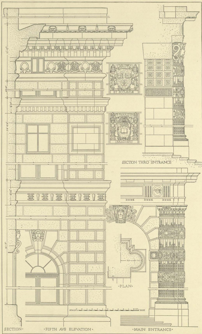
DETAILS OF EXTERIOR STONEMWORK UNIVERSITY CLUB, NEW YORK CITY. 1900
