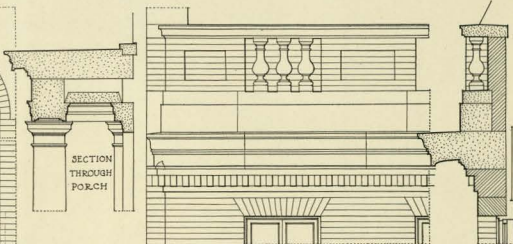
ELEVATION AND SECTION - MAIN CORNICE
