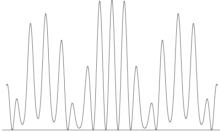
FIGURE 1.2. Intensity plot for a horizontal line across the bottom of Figure 1.1
