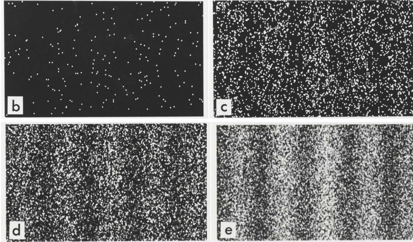
FIGURE 1.4. Four images from the 1989 experiment at Hitachi, showing the impact of individual electrons gradually building up to form an interference pattern. Image by Akira Tonomura and Wikimedia Commons user Belsazar. File is licensed under the Creative Commons Attribution-Share Alike 3.0 Unported license.
