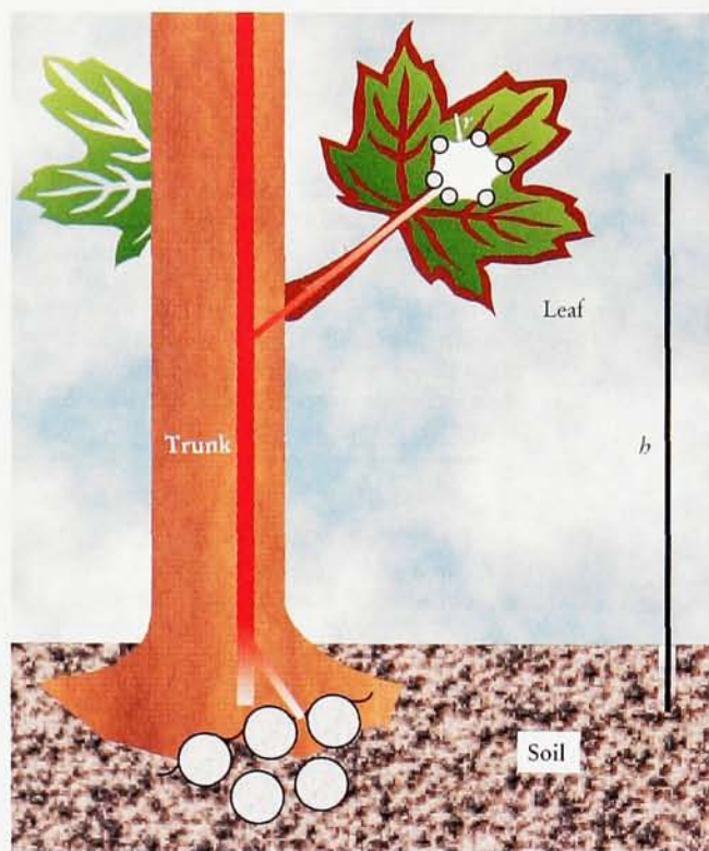
FIGURE 4. CONTINUOUS COLUMNS OF LIQUID SAP, nearly pure water, run up a tree and connect the water between soil particles with the wet walls of the cells within the leaves that contact the air. Supporting the columns of height b , as well as offsetting the pressure losses due to flow and capillary forces within the soil, requires that the radius of curvature r of the final air-water interfaces be very small.
