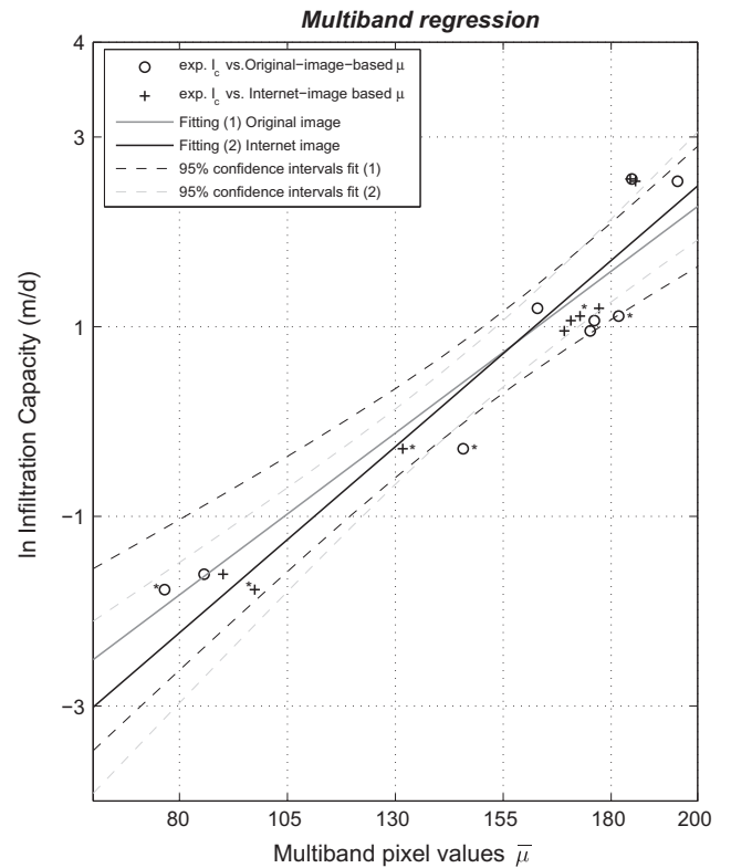
Fig. 6. Linear fitting of the experimental tests of the infiltration capacity (I c , in natural log scale) versus the multiband weighted average pixel values (μ̄), calculated at the 3 × 3 window around the S j experimental site. Weights are given by the relative quality of the information, based on the multiband window variances σ μ j,̄X 2 – see text. The region of confidence is expressed by the 95% confidence boundaries.
