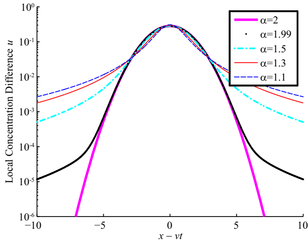
FIG. 1: (Color Online) The conservative component u(x, t) with a delta initial condition for various values of \alpha for K = 0.1 and at t = 1/D_\alpha .
