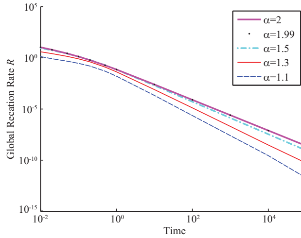
FIG. 4: (Color Online) The global reaction rate R against time for various values of \alpha and K = 0.1 .
