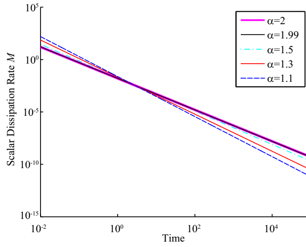
FIG. 3: (Color Online) The scalar dissipation M against time for various values of \alpha .
