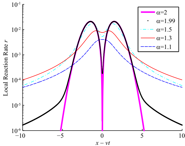
FIG. 2: (Color Online) Local reaction rate r with a delta initial condition for u for various values of \alpha at t = 1/D_\alpha and K = 0.1 .
