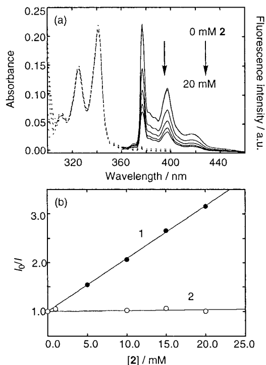
Figure 5. (a) UV-vis and fluorescence spectra of 1-methylpyrene upon the addition of 2 in 95% methanol/5% water (v/v): [1-methylpyrene] = 50.0 \mu\text{M} and [ 2 ] = 0–20 mM; (b) Stern-Volmer plots, (1) [BTA] = 0.0 mM and (2) [BTA] = 40.0 mM.
