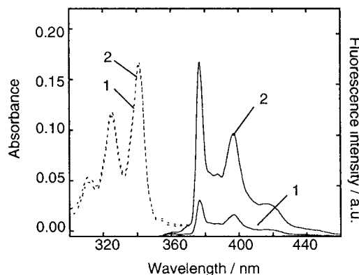
Figure 4. UV-vis and fluorescence spectra of 1 in 95% methanol/5% water (v/v): [ 1 ] = 1.05 \mu M when (1) [BTA] = 0.0 mM and (2) [BTA] = 1.0 mM; BTA, benzyltrimethylammonium hydroxide.
