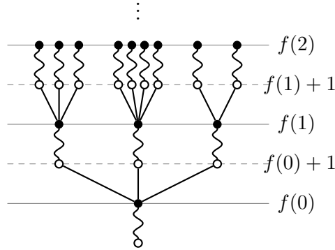
FIGURE 2.1. A strong subtree S of a tree T , with level function f . The circles represent nodes in T ; the solid circles in S , the hollow circles are in T \setminus S . The levels of S are included in the levels of T ; solid gray horizontal lines represent levels in S , dashed gray horizontal lines levels in T \setminus S . A node connected to another below it by a straight black line denotes a direct extension in T . Wavy lines indicate omitted (skipped over) portions of T . Note that all branchings are preserved: a nodes in S has the same number of direct extensions in S as in T .
