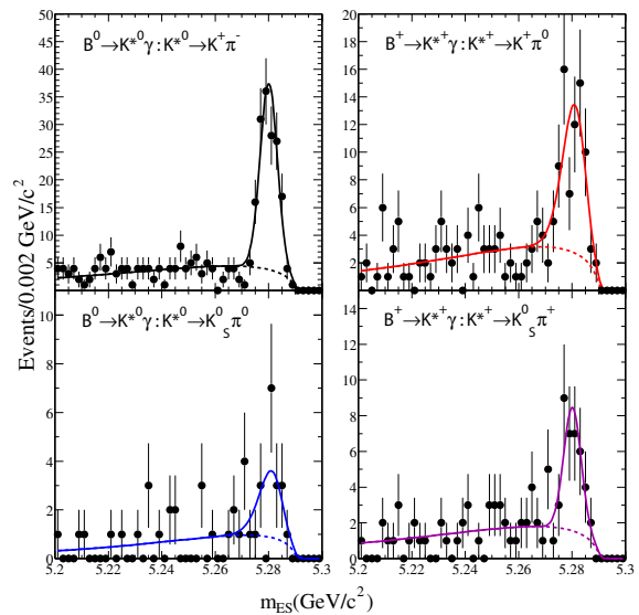
FIG. 2: m_{ES} for the B \rightarrow K^* \gamma candidates. The solid and dashed curves show respectively the fitted signal-plus-background and the background alone. The fits used to extract the signal yield are described in the text.
