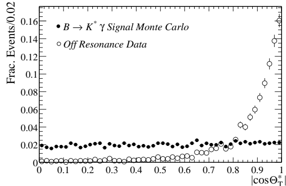
FIG. 1: The event shape variable |\cos \theta_T^*| for B^0 \rightarrow K^{*0} \gamma , K^{*0} \rightarrow K^+ \pi^- Monte Carlo and off-resonance data.
