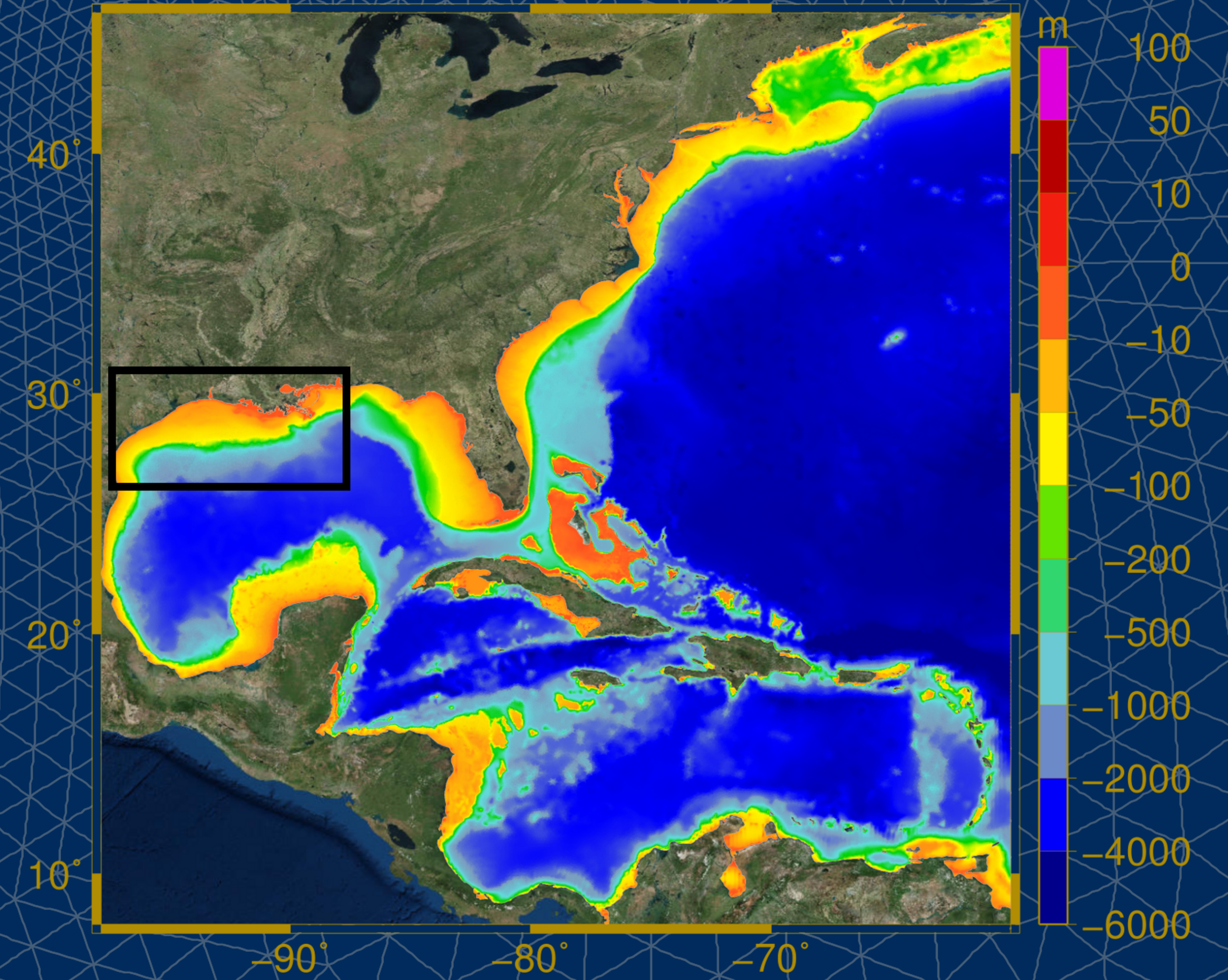
Bathymetry / Topography
