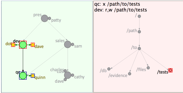
Figure 3: Role Node Highlight with Children
