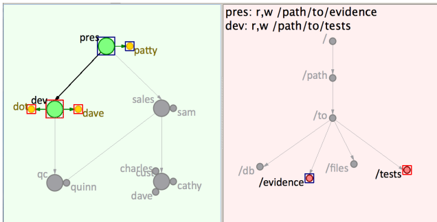
Figure 4: Role Node Highlight with Parents
