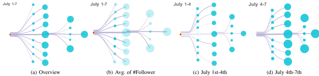
Fig. 10: Eiffel visualization on Higgs social influence graph.
