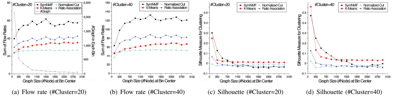
Fig. 1: Performance of node summarization algorithms on AMiner V8 citation influence graphs. To reduce the experimental data volume, only papers on the visualization topic were considered.
