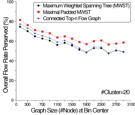
Fig. 2: Edge summarization performance measured by the percentage of flow rate preserved from the IGS after node summarization (larger is better). The experimental setting is the same as that in Figure 1.
