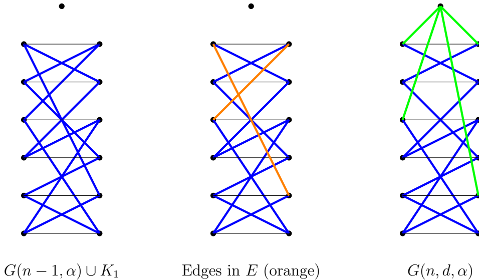
Figure 5: Illustration of some aspects of the construction when n is odd.
