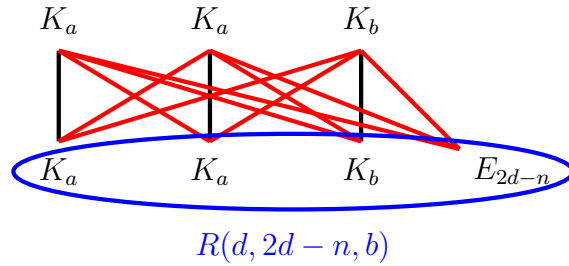
Figure 8: Construction when n/2 \leq d \lesssim n (black lines represent perfect matchings and red lines represent complete bipartite graphs).
