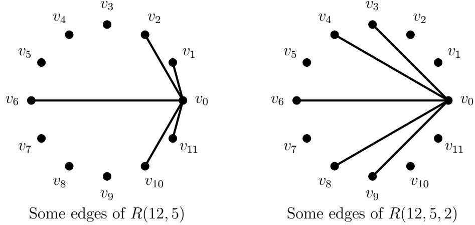
Figure 6: The edges of R(12, 5) and R(12, 5, 2) that are incident with v_0 .
