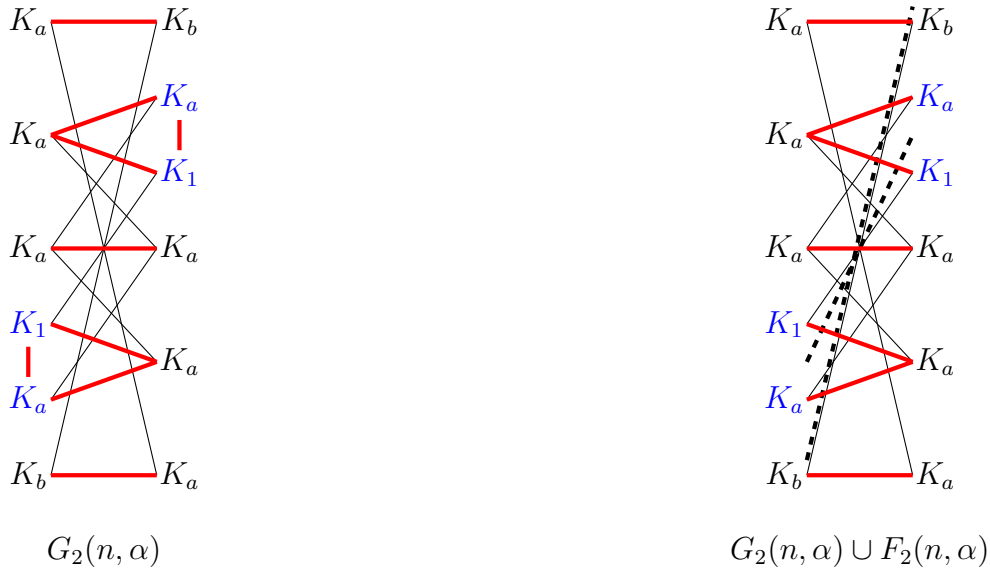
Figure 4: Illustration of some aspects of the construction when b = a + 1, n_a = n_b + 1, n even.
