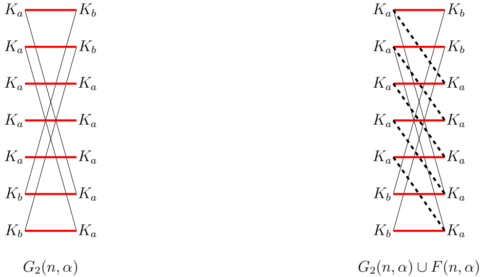
Figure 2: Illustration of some aspects of the construction when n_a > n_b , b = a - 1 , n even.
