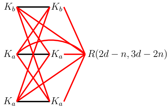
Figure 7: Construction when d \gtrsim 2n/3 (black lines represent perfect matchings and red lines represent complete bipartite graphs).
