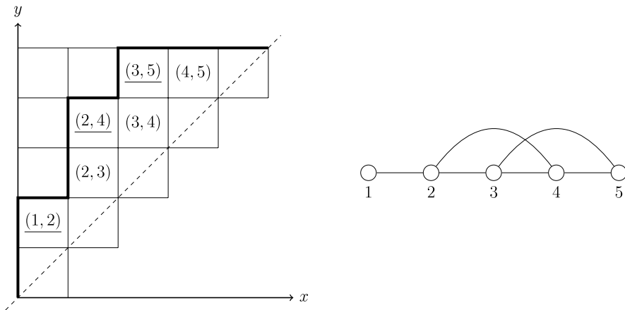
Fig. 2. The staircase path of w and the graph H_w for w = xxDxxDxDxDDD .
