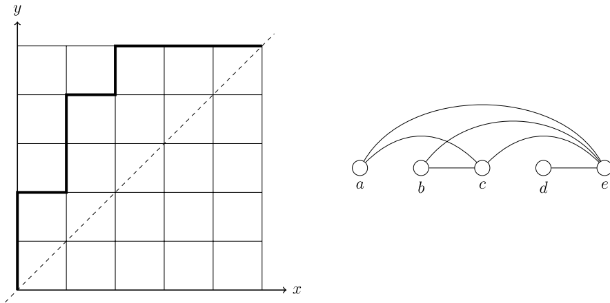
Fig. 1. The Dyck path corresponding to the Dyck word w = xxDxxDxDDD and the associated graph G_w .
