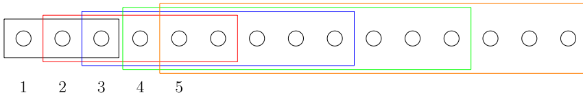
Fig. 5. The graph H(5, 3) .
