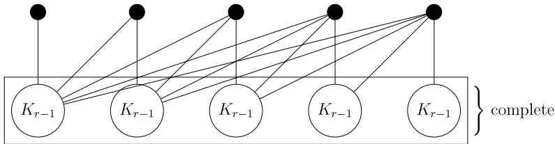
Fig. 4. The graph G(5, r) . An edge from a vertex on top to a K_{r-1} below indicates that the vertex on top is joined to all vertices of K_{r-1} .
