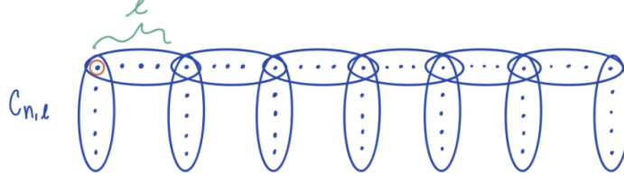
Figure 4: The linear uniform hypercomb C_{6,5} .
