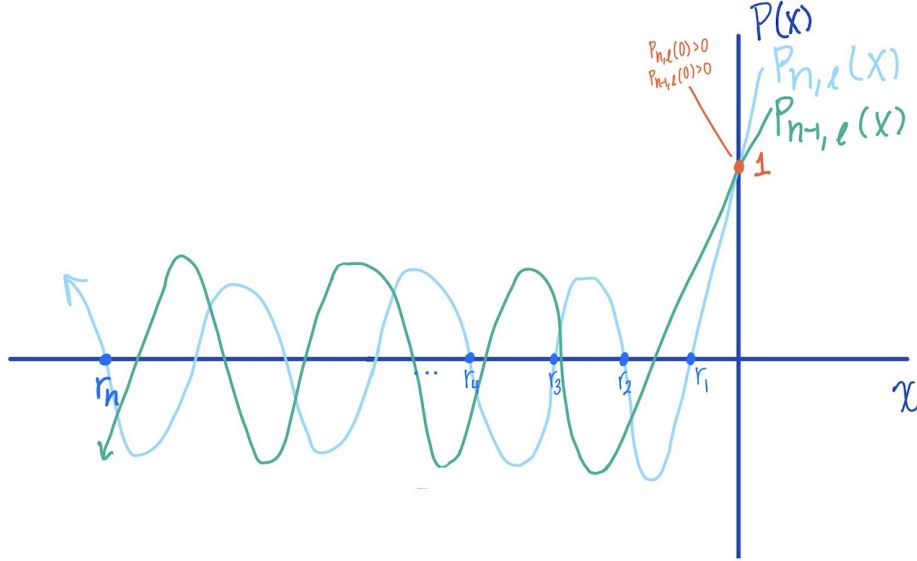
Figure 3: The inductive relationship between P_{n,\ell} and P_{n-1,\ell} .
