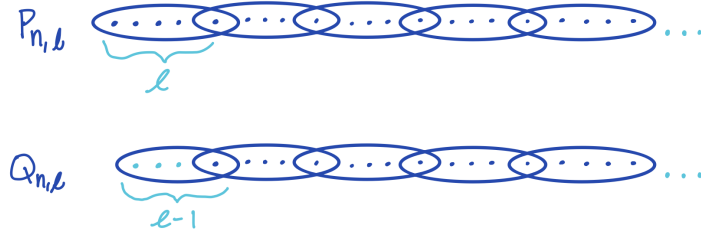
Figure 1: The linear hyperpaths P_{n,\ell} (top) and Q_{n,\ell} (bottom).
