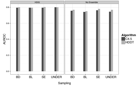
Fig. 3. Batch average results in terms of computational AUROC (higher is better) using different sampling strategies and batch-ensemble weighting methods with C4.5 and HDDT over all drifting MOA datasets .
