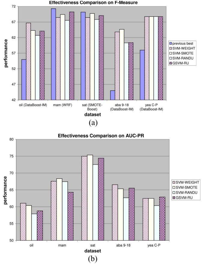
Fig. 10. (a) F -measure analysis. (b) AUC-PR analysis.
