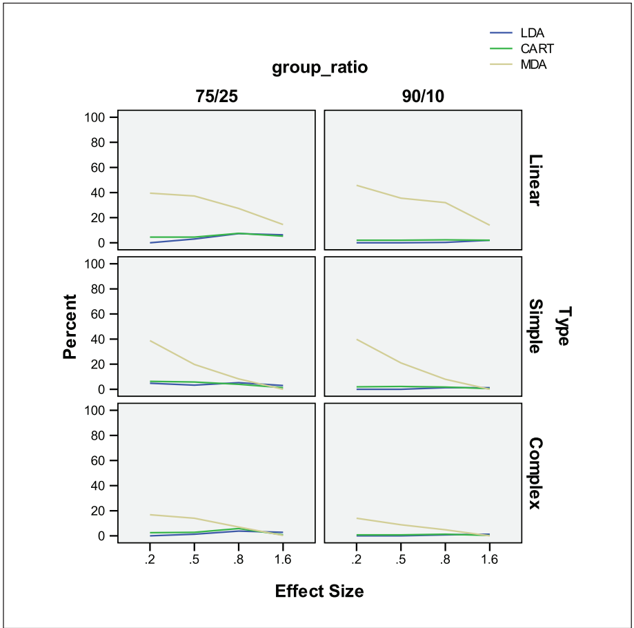
Figure 2. Large-group misclassification percentages for LDA, CART, and MDA by effect size, sample size ratio, and type of underlying model Note. LDA = linear discriminant analysis; CART = classification and regression trees; MDA = mixture discriminant analysis.
