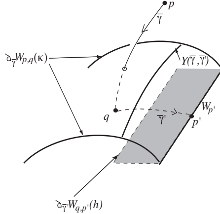
Fig. 4.13. The structure of M_p^- near W_p^- .
