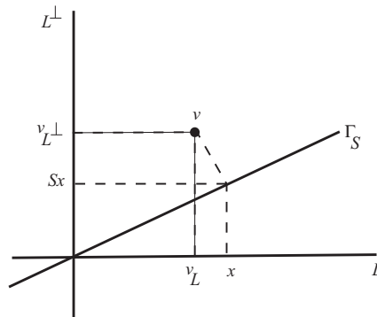
Fig. 6.5. Subspaces as graphs of linear operators.
