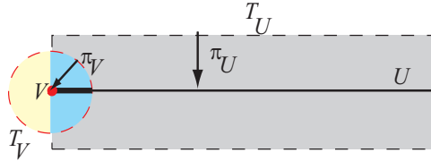
Fig. 4.5. Non-compatible tubular neighborhoods
