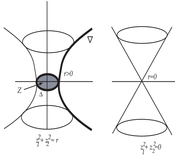
Fig. 5.4. The vanishing cycle for functions of n = 2 variables.
