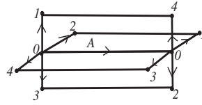
Fig. 4.4. A surface with a codimension 1 singularity.
