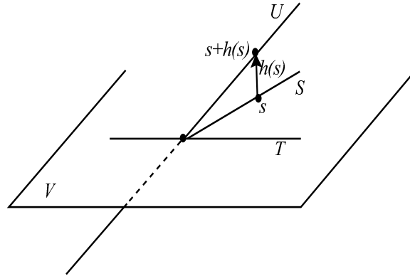
Fig. 4.1. Computing the gap between two subspaces.
