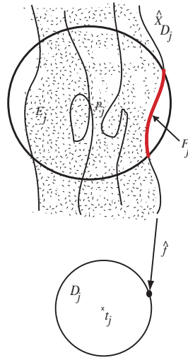
Fig. 5.3. Isolating the critical points.
