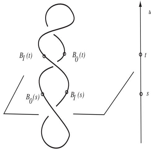
Fig. 6.2. Unwinding a garden hose.
