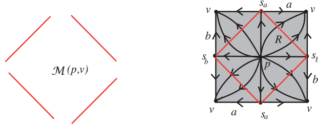
Fig. 4.11. A Morse-Smale flow on the 2-torus and the spaces of broken tunnelings.
