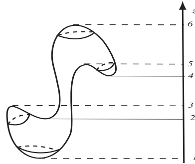
Fig. 6.3. An embedding of S^2 in \mathbb{R}^3 .
