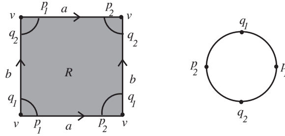
Fig. 4.7. A Whitney stratification of the 2-torus.
