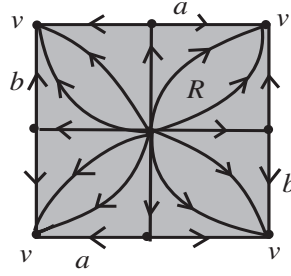
Fig. 4.10. A Morse-Smale flow on the 2-torus.
