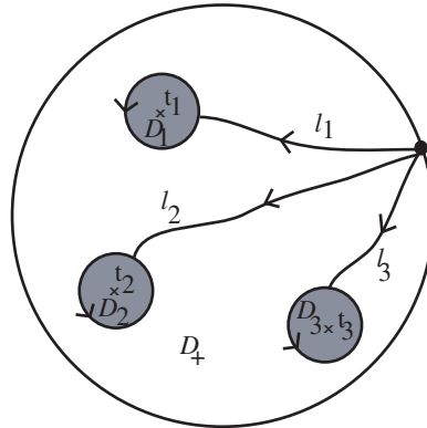
Fig. 5.2. Isolating the critical values.
