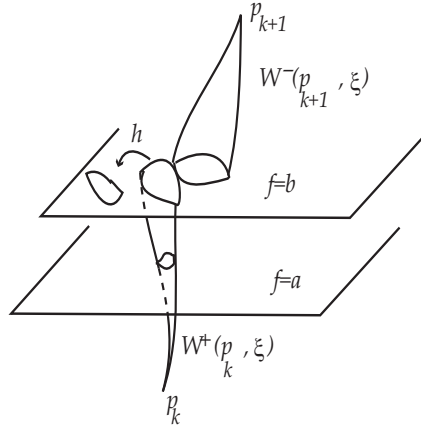
Fig. 2.14. Deforming a gradient-like flow.
