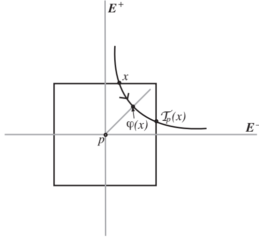
Fig. 4.12. The block \mathcal{B}_p(\varepsilon) and the tunneling map \mathcal{J}_p .
