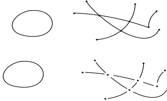
Fig. 4.14. The link \mathcal{L}_{p,p'} (top half) and its blowup along the 0-strata (bottom half).
