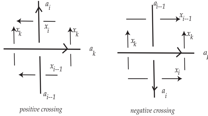
Fig. 2.3. The Wirtinger relations.
