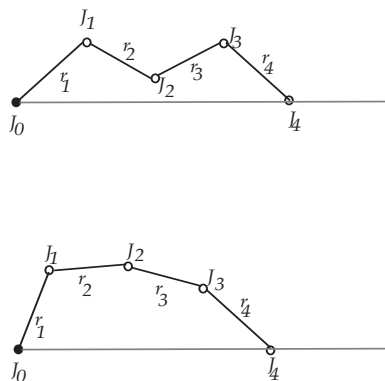
Fig. 1.2. A robot arm with four segments.
