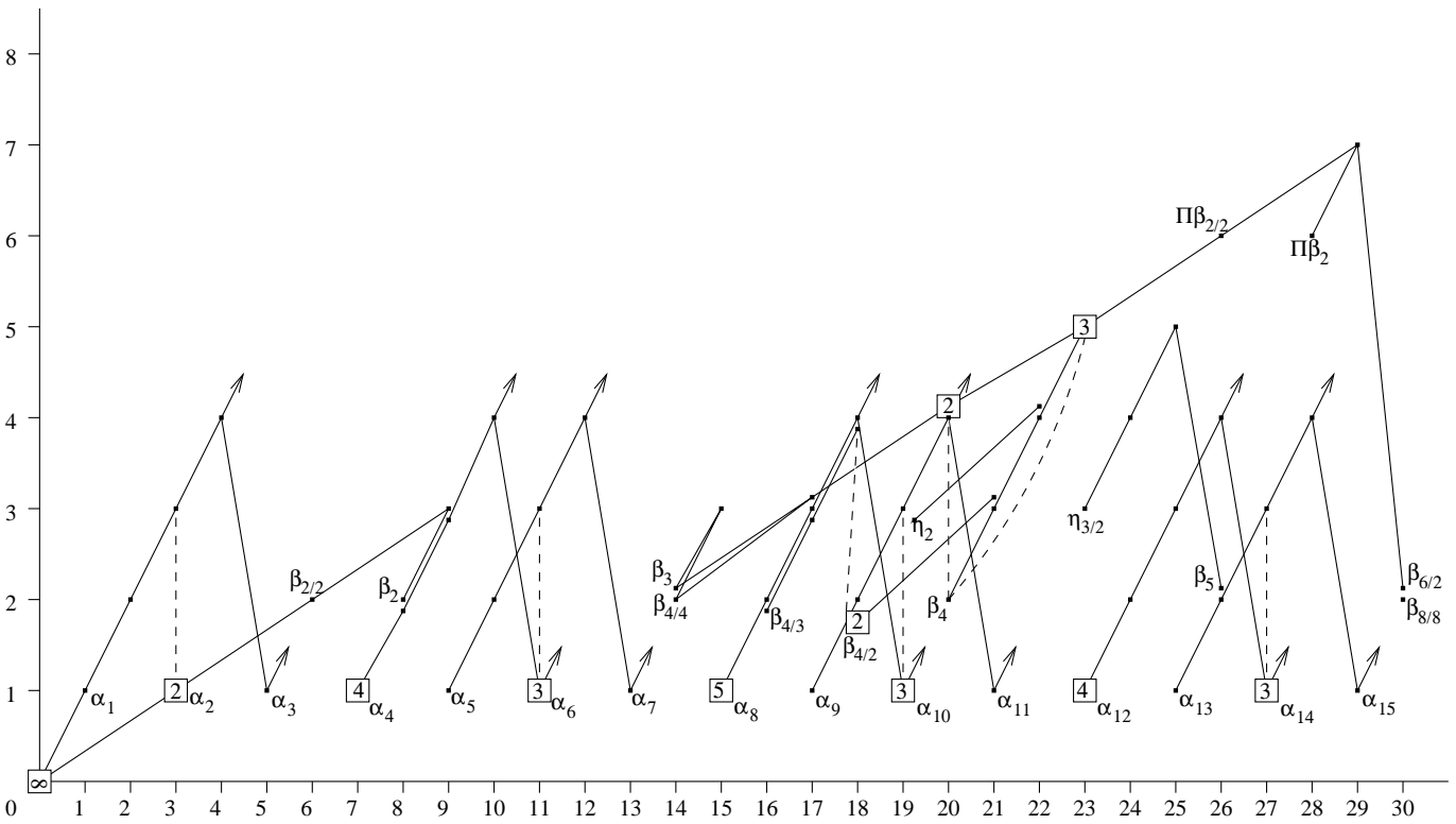
Figure 1: The Adams-Novikov spectral sequence at p = 2 .
