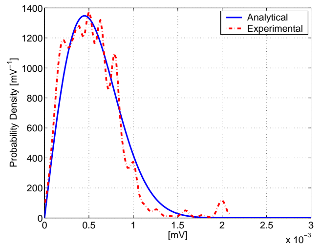
Figure 11: Rayleigh Fading with MICAz hardware: there remains a line-of-sight path, but it is comparable to a number of other multipath components.
