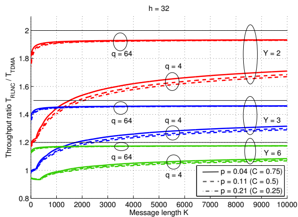
Fig. 14. Throughput ratio T_{\text{RLNC}}/T_{\text{TDMA}} for RLNC and different values of p .
