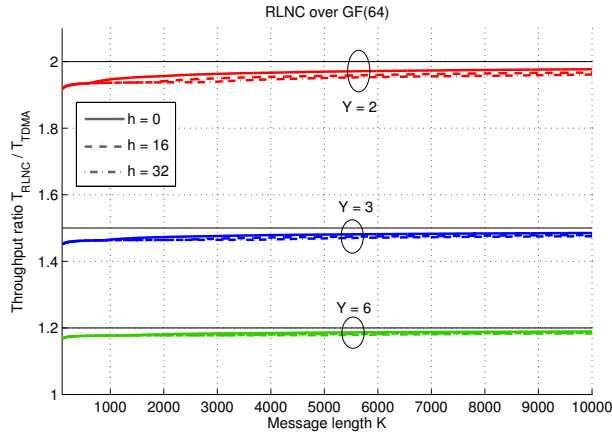
Fig. 11. Average throughput ratio T_{\text{RLNC}}/T_{\text{TDMA}} for GF(64).
