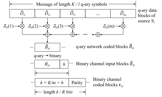
Fig. 2. A source S_i divides its message of length K bits into m blocks. RLNC over GF(q) is then used to create q -ary network coded blocks \tilde{B}_{ib} . After q -ary to binary conversion, a header of size h bits is appended to each block and the resulting block of size k = K/m + h bits is protected by a linear channel code of rate R to create binary channel coded blocks v_{ib} .
