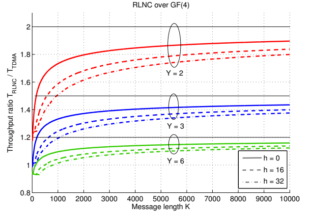
Fig. 10. Average throughput ratio T_{\text{RLNC}}/T_{\text{TDMA}} for GF(4).
