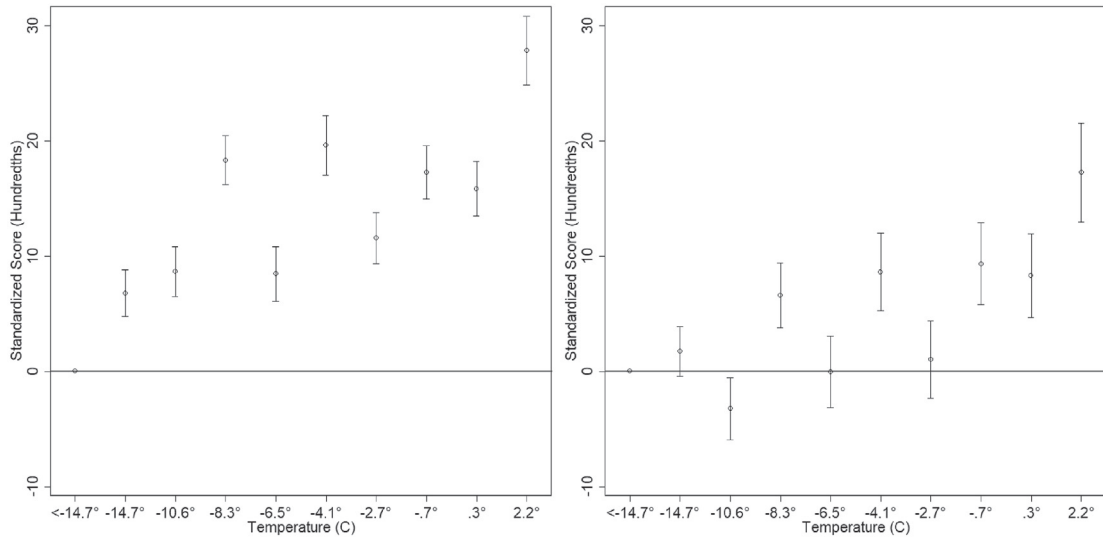
Fig. A1 Temperature and Performance (Deciles).
