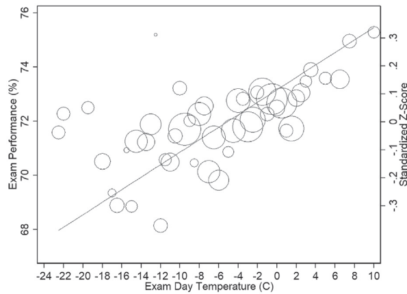
Fig. 2. Temperature and Performance (Only Year Controls). In this figure, we plot the imputed residual exam grade (after accounting for year fixed effects) by exam day temperature. Temperature is rounded to the nearest 0.5 °C. Markers are sized proportional to number of observations they represent.
