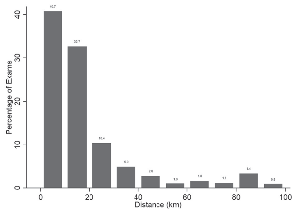
Fig. A4 Distance to Student Address.
