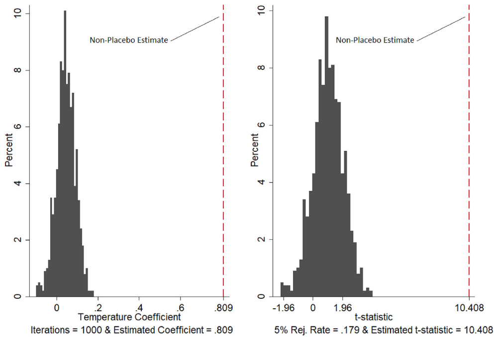
Fig. 6. Placebo. In this figure, we present histograms of the estimated temperature coefficients and associated t-statistics for a placebo exam day temperature. Placebo temperatures are randomized within-student and without replacement. If an exam was assigned a placebo temperature from the same exam season, that observation was dropped. The preferred specification in Table 2 was run 1000 times. A reference line corresponding to our preferred specification, on the correct exam day temperature, is provided in each panel.
