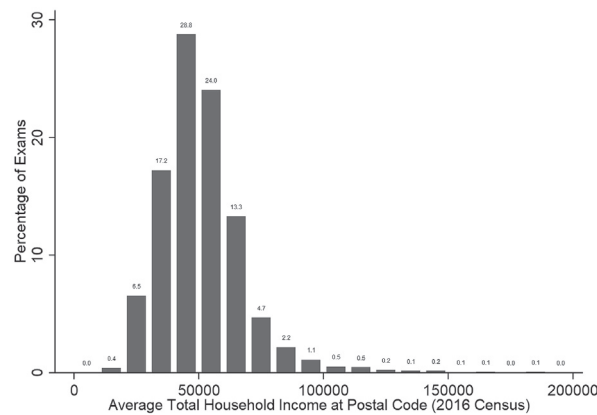
Fig. A5 Student Application Address Average Income.
