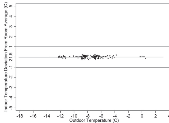
Fig. 4. Indoor and Outdoor Temperatures (MNT021). In this figure, we plot the outdoor temperatures realized during 2018 December exams and the internal temperature variations from room average in the largest exam room by contribution to sample. We fit a regression line with slope coefficient of 0.0003 and an associated t-statistic of 0.10. Reference lines are provided at 1 °C above and below room average.
