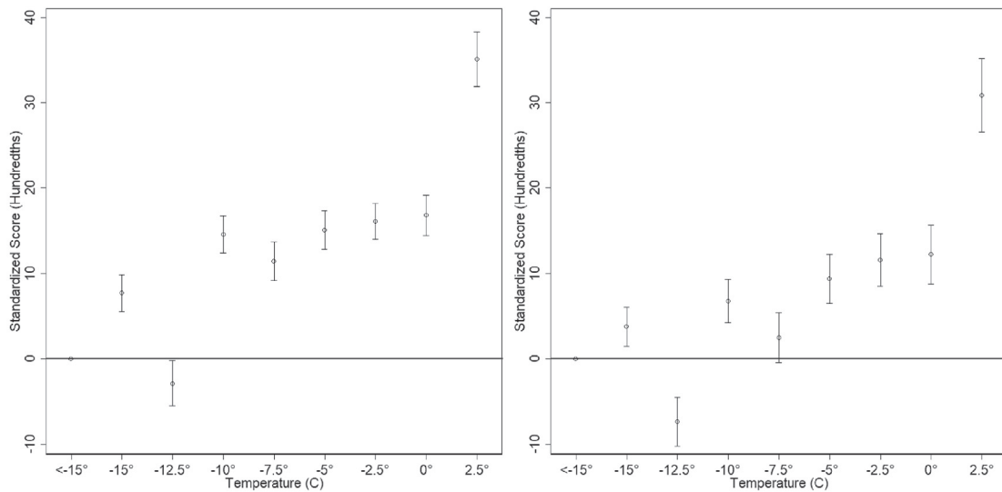
Fig. 3. Temperature and Performance (Non-Linear). In this figure, we present the estimated coefficients by “binning” daily temperatures into 2.5 °C intervals. The reference category is exams written with daily temperatures below -15^{\circ}\text{C} . The dependent variable is exam score standard deviations in hundredths. The left panel corresponds to a parsimonious specification with student and year fixed effects, precipitation, and its interaction with each temperature bin. The right panel corresponds to our preferred specification with additional controls. Whiskers indicate the 95% confidence level.
