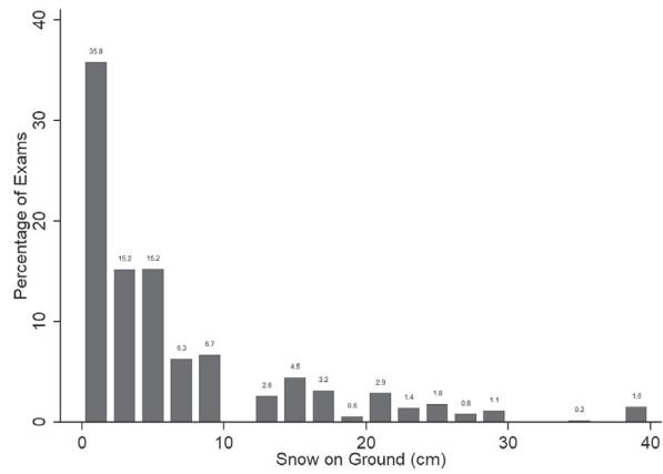
Fig. A3 Snow on Ground.
