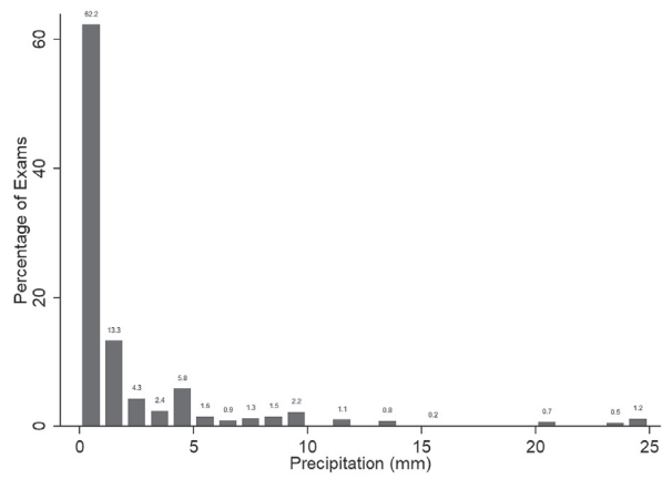
Fig. A2 Precipitation.
