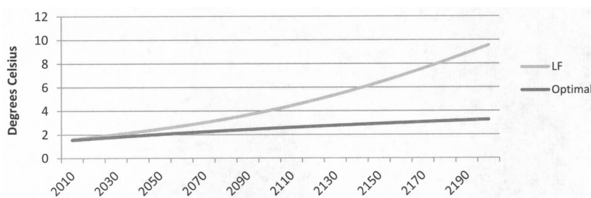
FIGURE 7.—Increases in global temperature: optimum versus laissez-faire.
