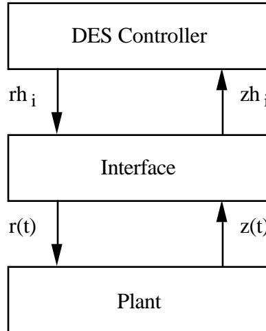
Figure 2. Hybrid Supervisory Control Architecture. The interface receives continuous measurements z(t) and issues a sequence of symbols \{z(i)\} which the DES controller processes to issue a sequence of control symbols \{r(i)\} . These are translated by the interface to (piecewise) continuous input commands r(t) .
