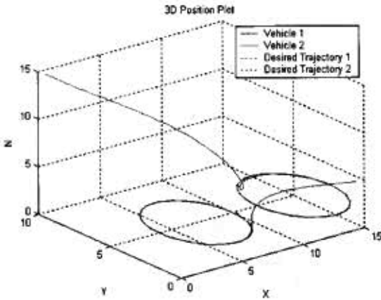
Figure 6: Two-Vehicle Simulation with Sufficient Vehicle Velocities
