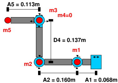
Figure 3. Pioneer 3 Arm
