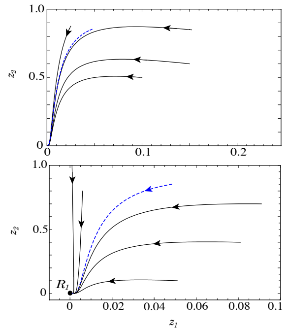
Fig. 4. The dashed line represents the calculated MEPT and the thin lines represent trajectories. The top panel is identical to Fig. (4) in [3], while the bottom panel is a closer look with a different set of trajectories is illustrated. R_1 represent the physical equilibrium state of the system.
