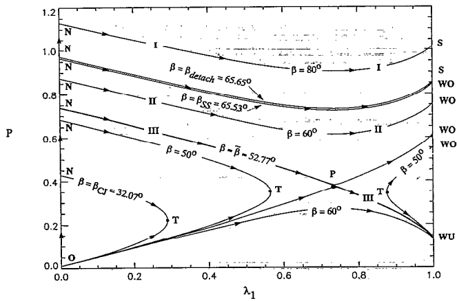
FIG. 3. P_1, \lambda_1 phase plane.
