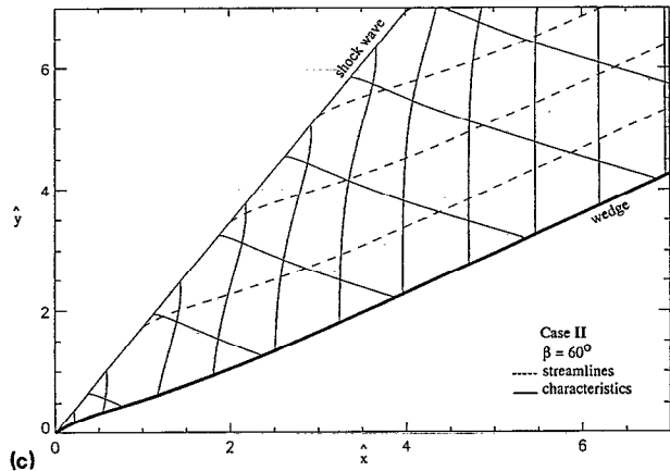
FIG. 6. (a) Predictions of the reaction progress variables for a weak overdriven oblique detonation. (b) Predictions of pressure for a weak overdriven oblique detonation. (c) Streamlines and characteristics for a weak overdriven oblique detonation.
