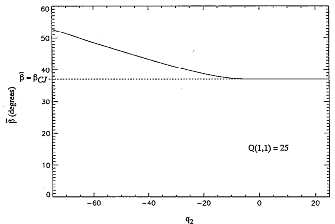
FIG. 8. Eigenvalue wave angle \tilde{\beta} as a function of heat released in second reaction q_2 with global heat release Q(1,1) held constant.
