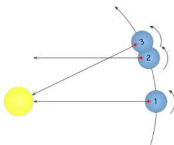
Figure 2. The Sidereal Day. At time 1, the Sun and a certain distant star are both overhead. At time 2, the planet has rotated 360^\circ and the distant star is overhead again ( 1 \rightarrow 2 = one sidereal day). But it is not until a little later, at time 3, that the Sun is overhead again ( 1 \rightarrow 3 = one solar day).
