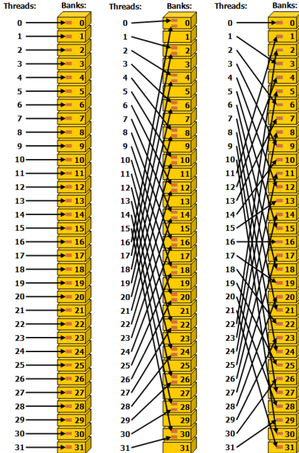
Left: Linear addressing with a stride of one 32-bit word (no bank conflict).
