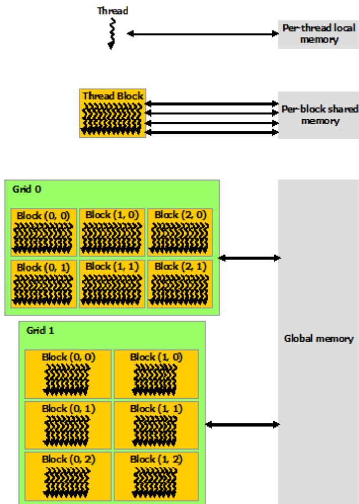
Figure 7 Memory Hierarchy
